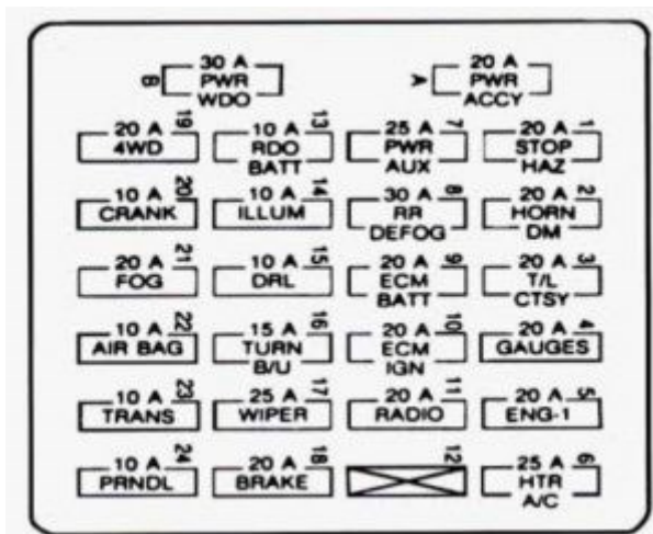
GMC Jimmy – fuse box diagram
