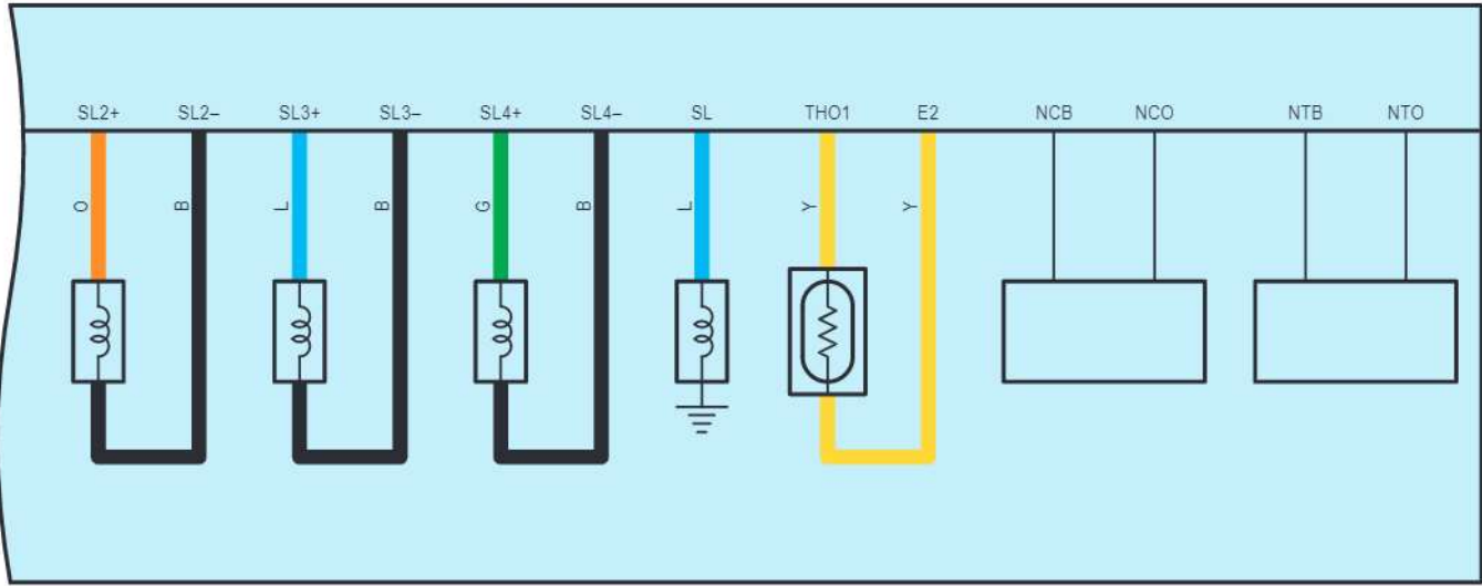
B52 Transmission Control ECU Assembly
