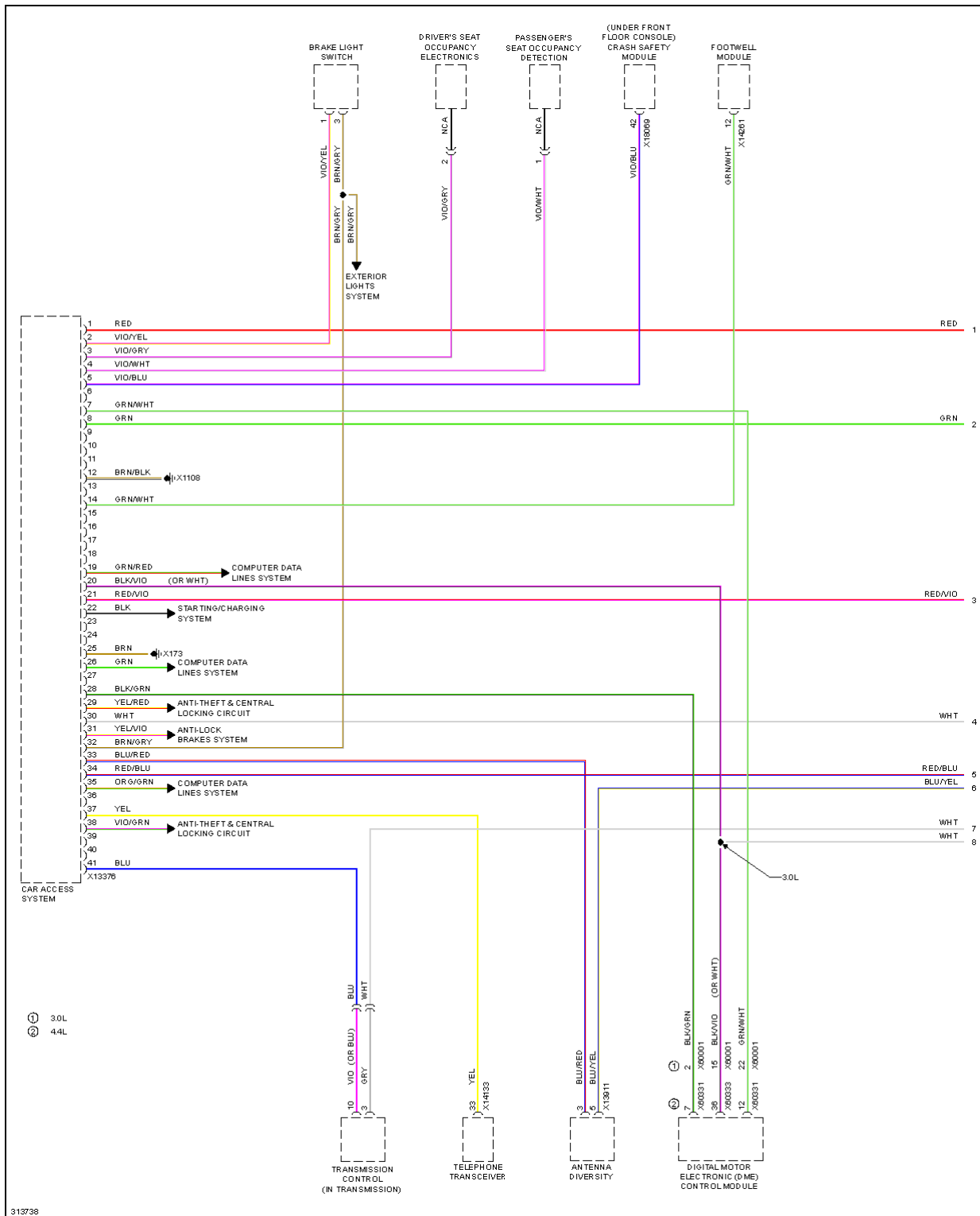
Fig. 14: Access/Start Circuit (1 of 3)
