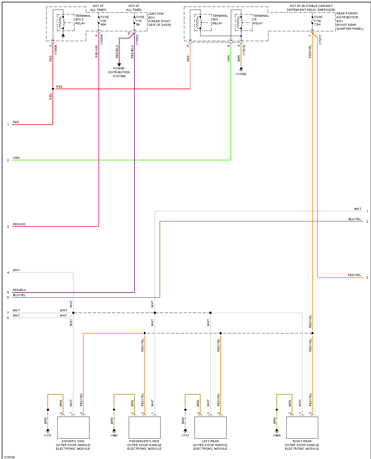
Fig. 15: Access/Start Circuit (2 of 3)
