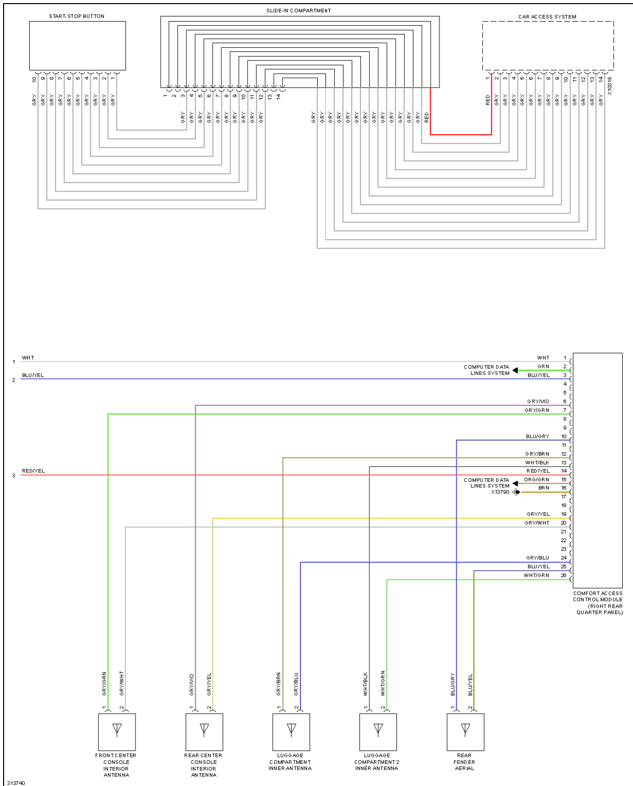
Fig. 16: Access/Start Circuit (3 of 3)
