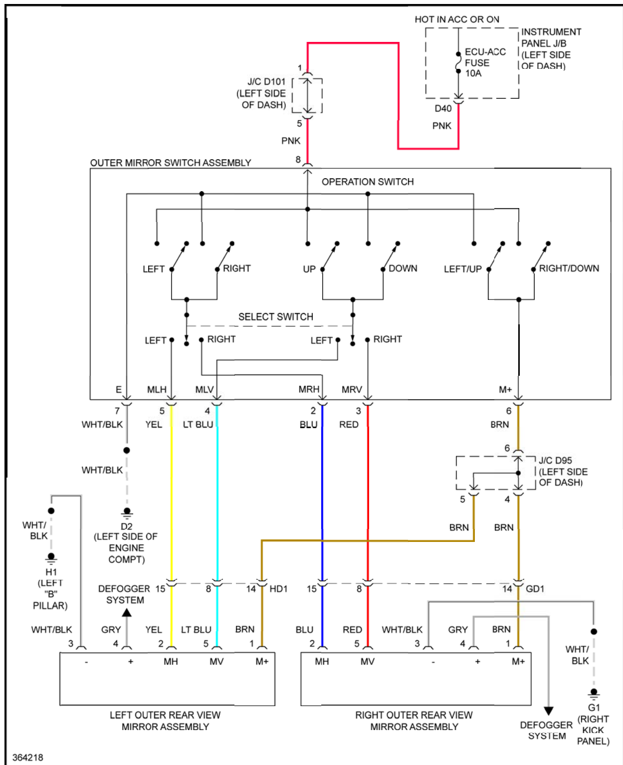
Fig. 81: Power Mirrors Circuit
