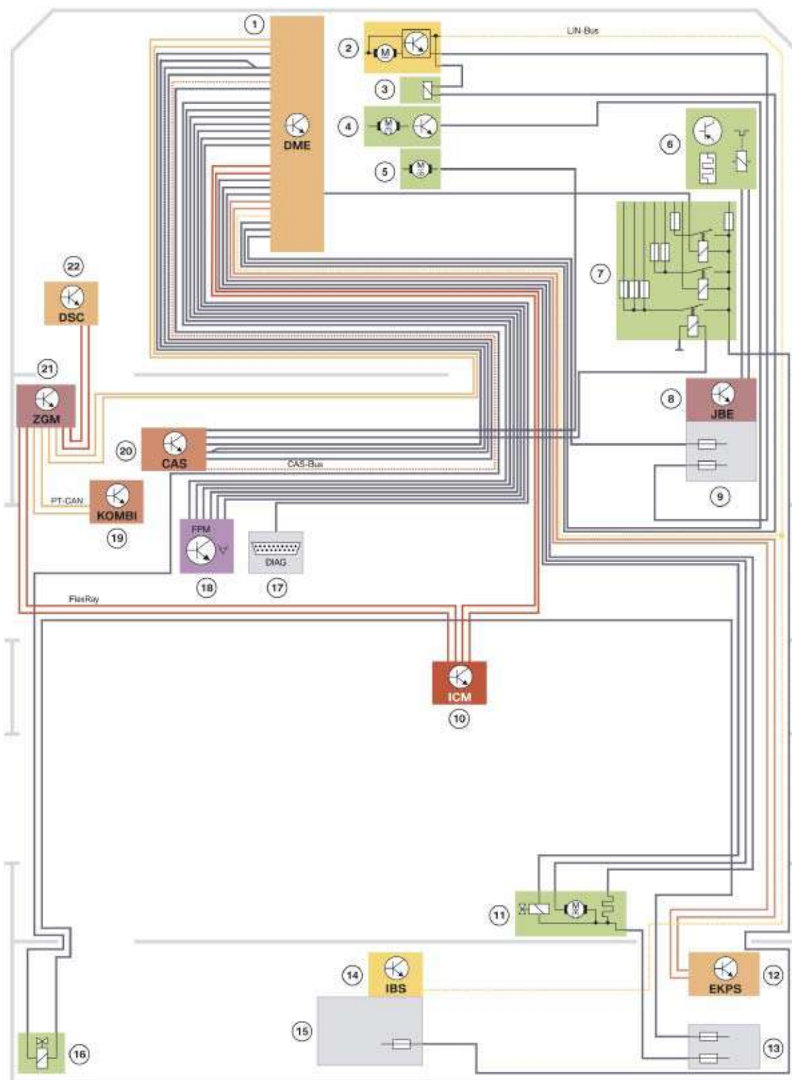
ISTA wiring schematic: SSP-BSB-T6109023 Motor interface N55
