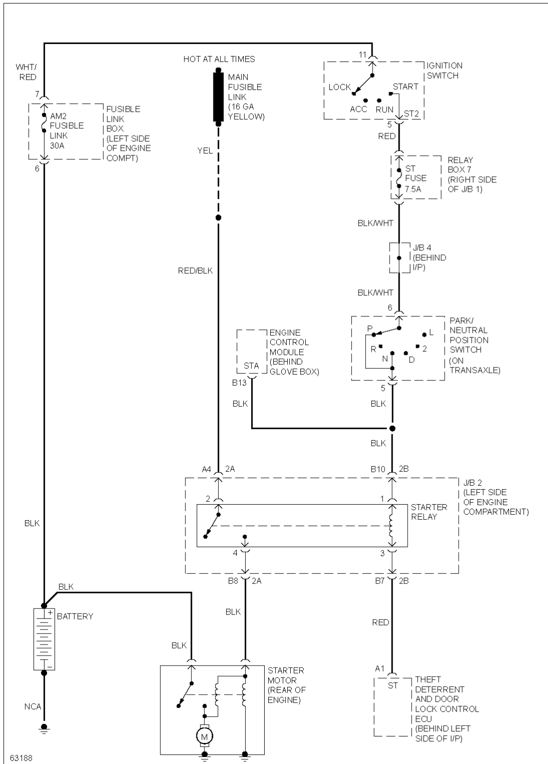
Fig. 56: Starting Circuit
