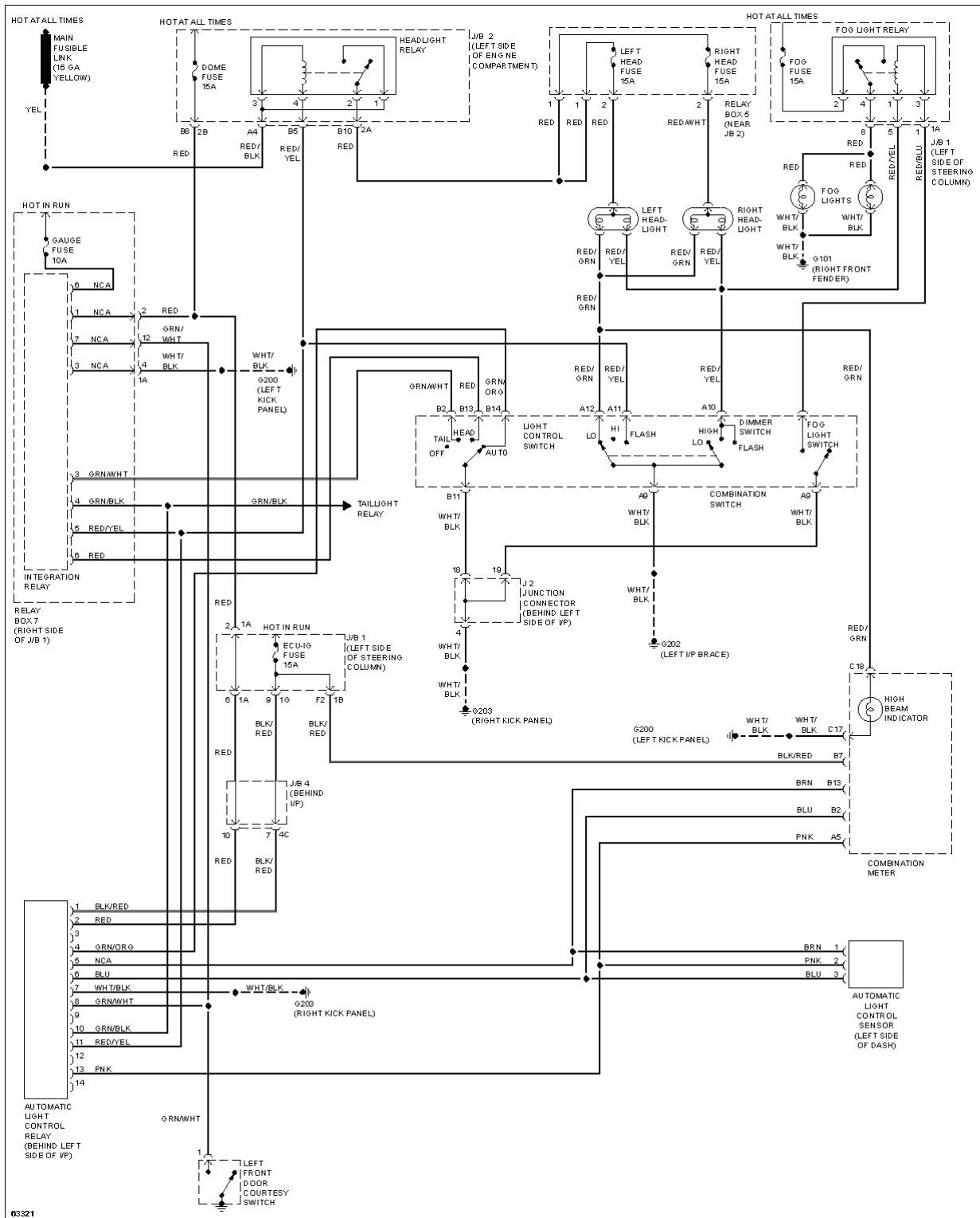
Fig. 27: Headlight Circuit, W/O DRL
