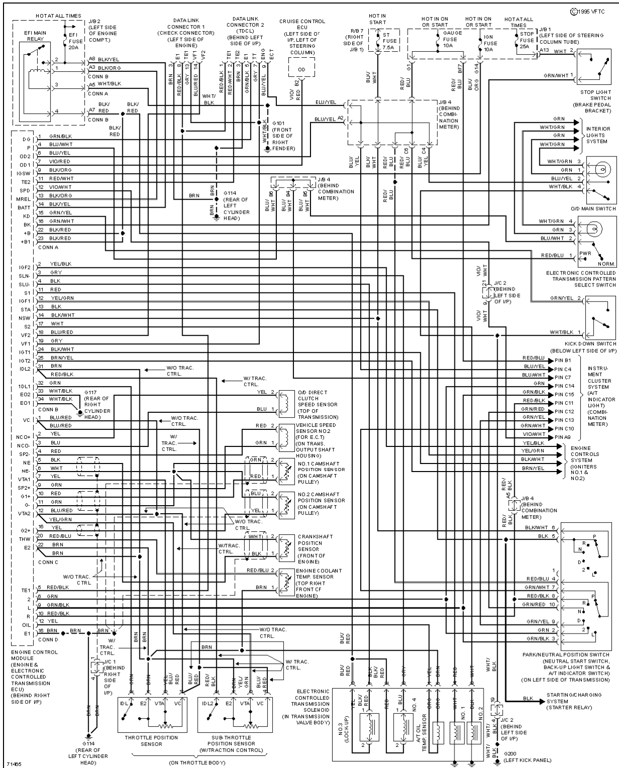
Fig. 58: Transmission Circuit
