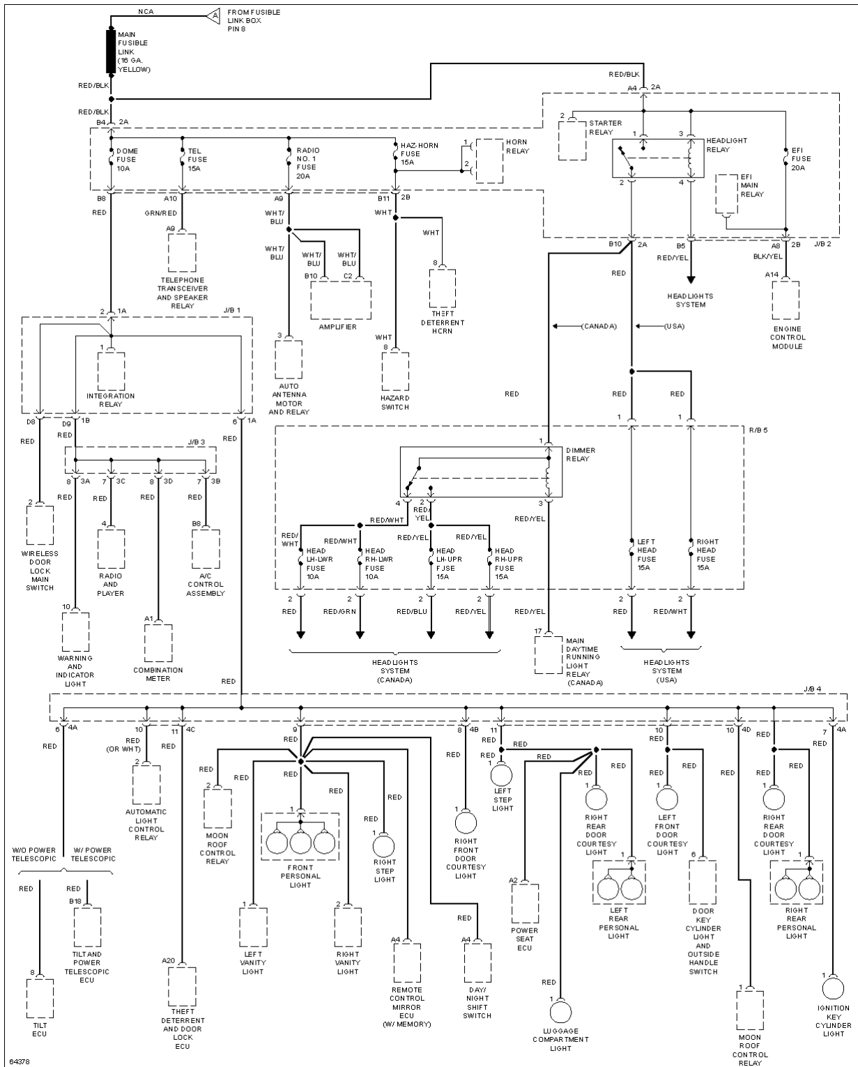
Fig. 43: Power Distribution Circuit (4 of 5)
