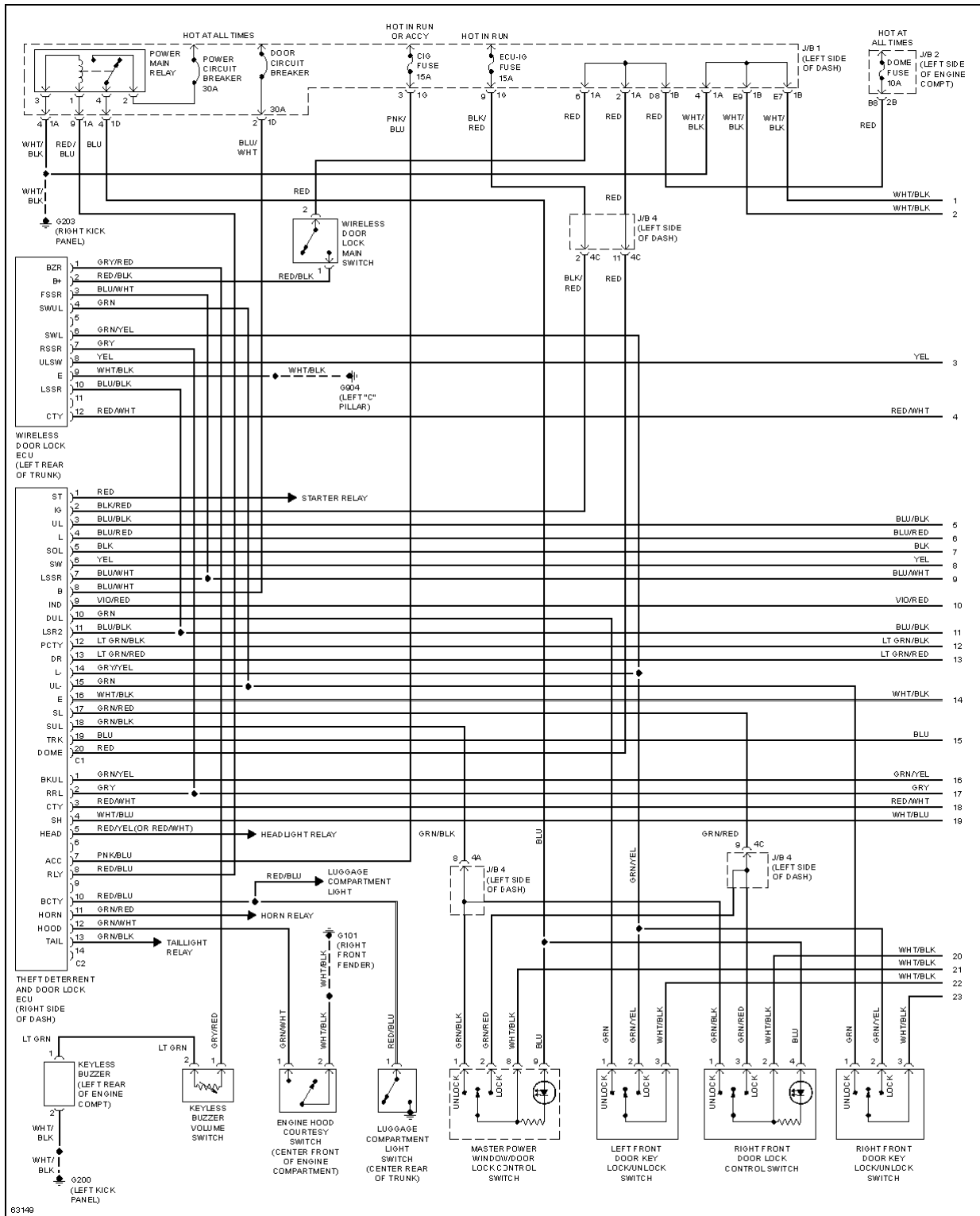
Fig. 45: Keyless Entry & Anti-Theft Circuit (1 of 2)
