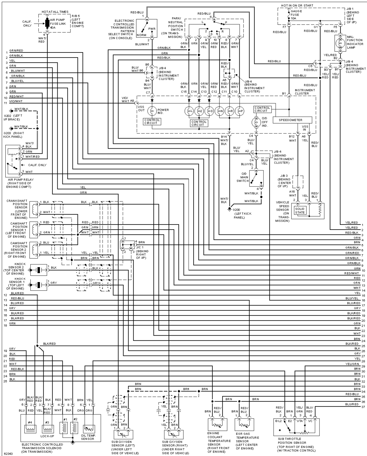
Fig. 17: 4.0L, Engine Performance Circuits (2 of 3)
