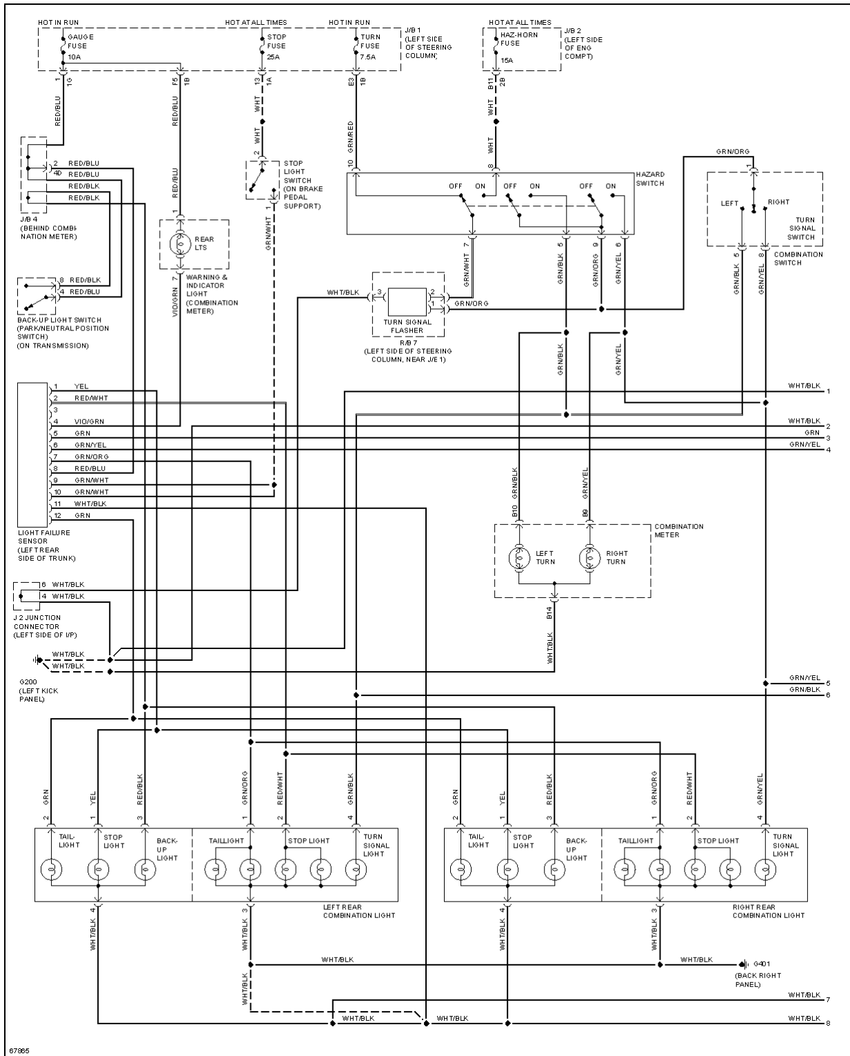
Fig. 19: Exterior Light Circuit (1 of 2)
