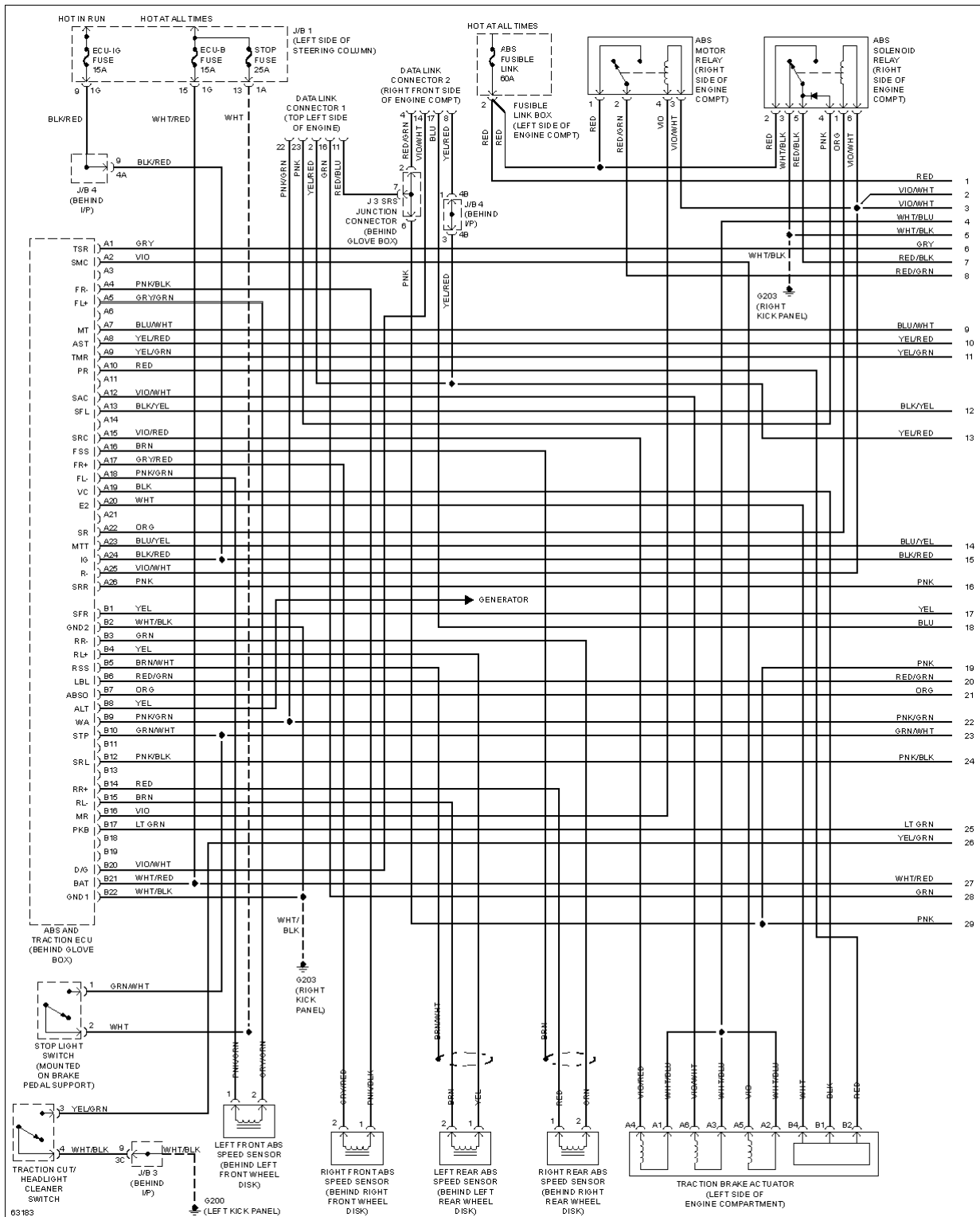
Fig. 4: Anti-lock Brake Circuits, W/ Traction Control (1 of 2)
