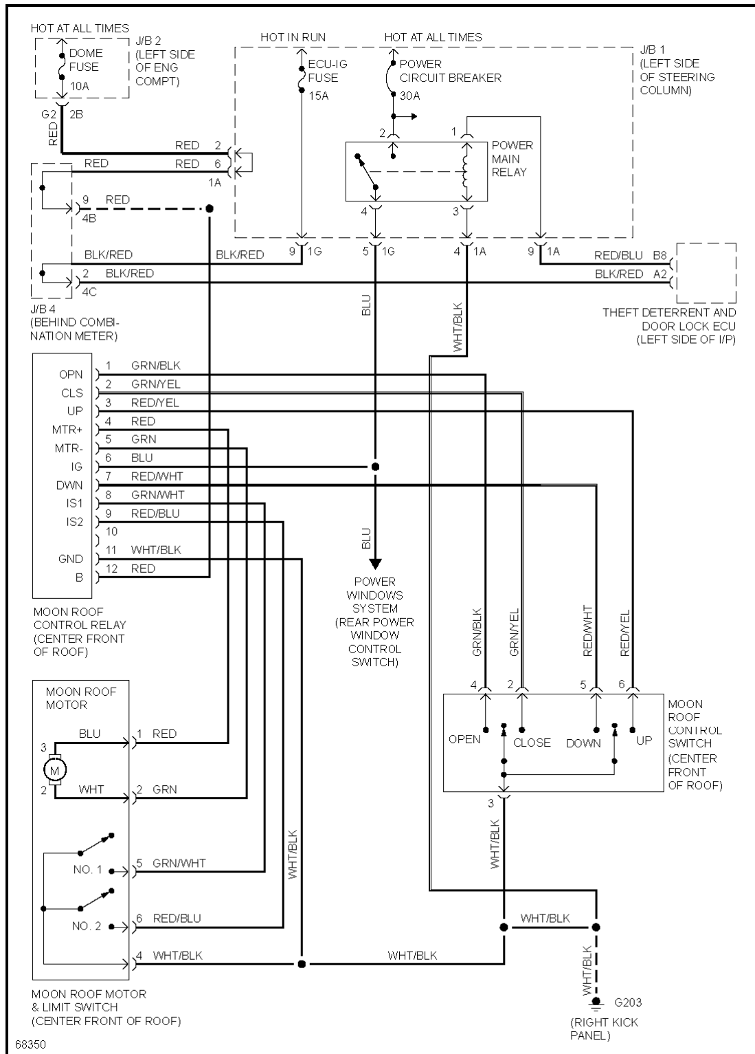
Fig. 50: Moonroof Circuit
