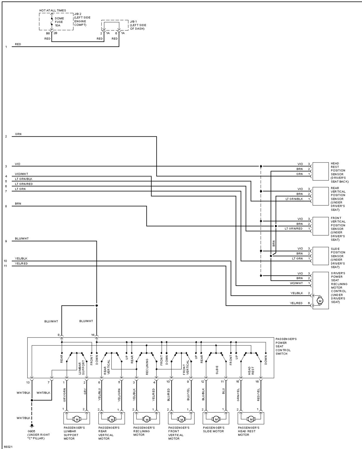
Fig. 36: Memory Seat Circuit (2 of 2)
