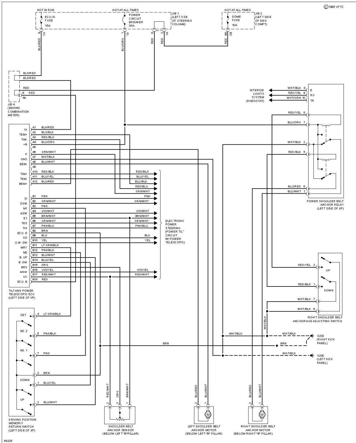
Fig. 38: Power Shoulder Belt Anchorage Circuit
