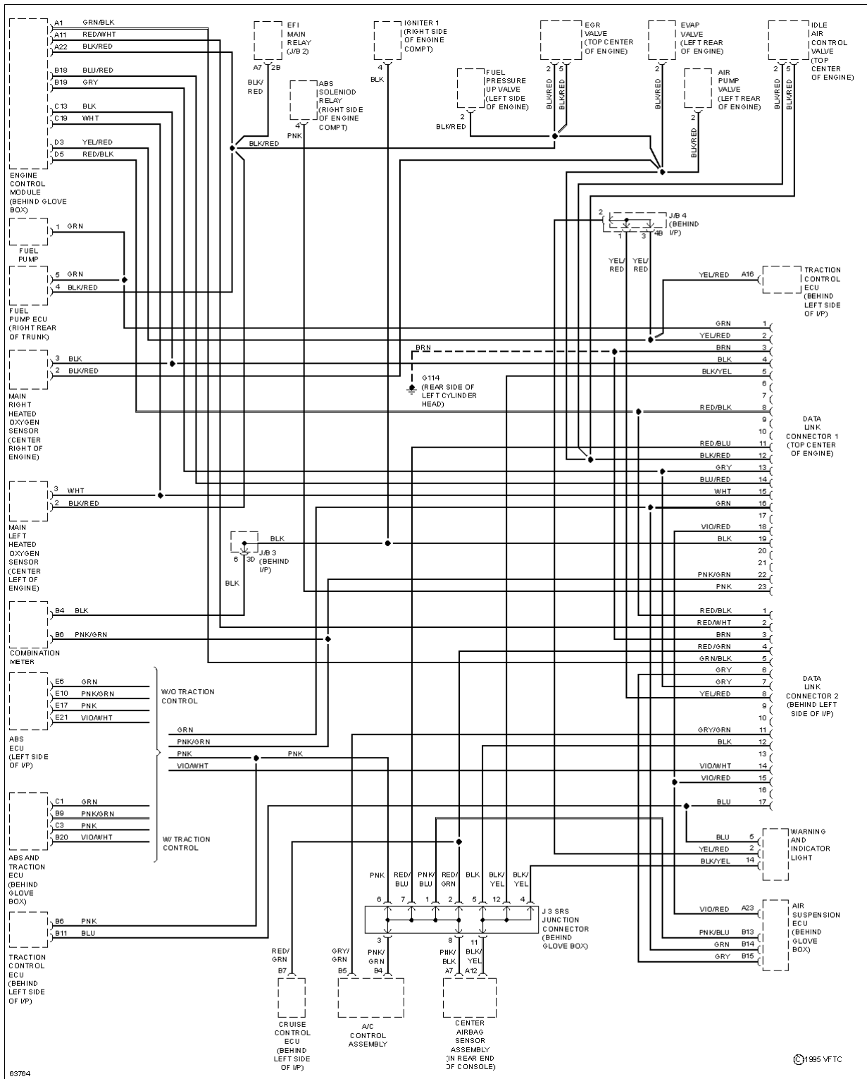
Fig. 8: Computer Data Lines
