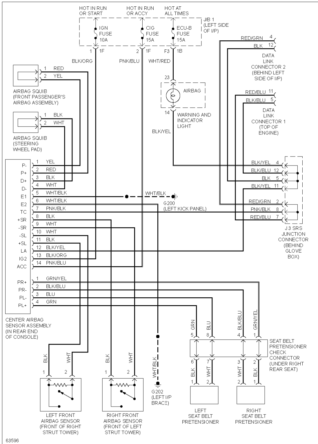
Fig. 57: Supplemental Restraint Circuit
