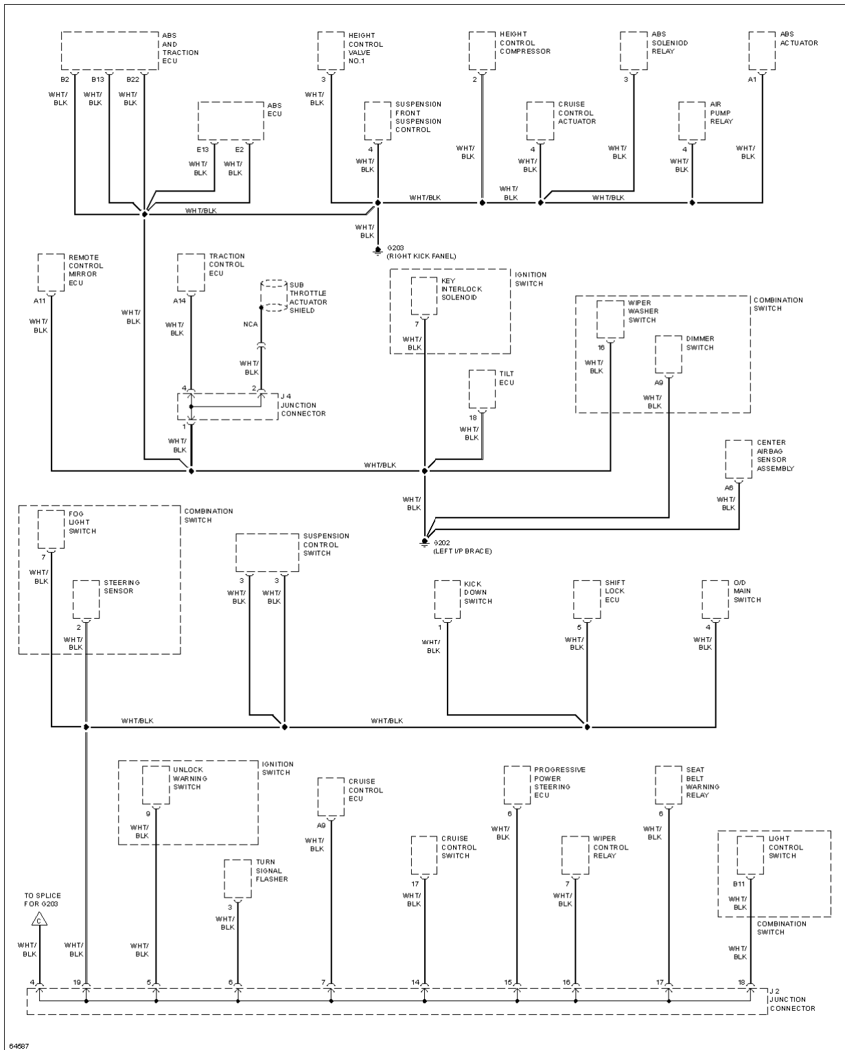
Fig. 24: Ground Distribution Circuit (4 of 5)
