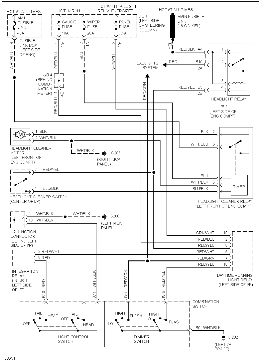
Fig. 62: Headlamp Washer Circuit
