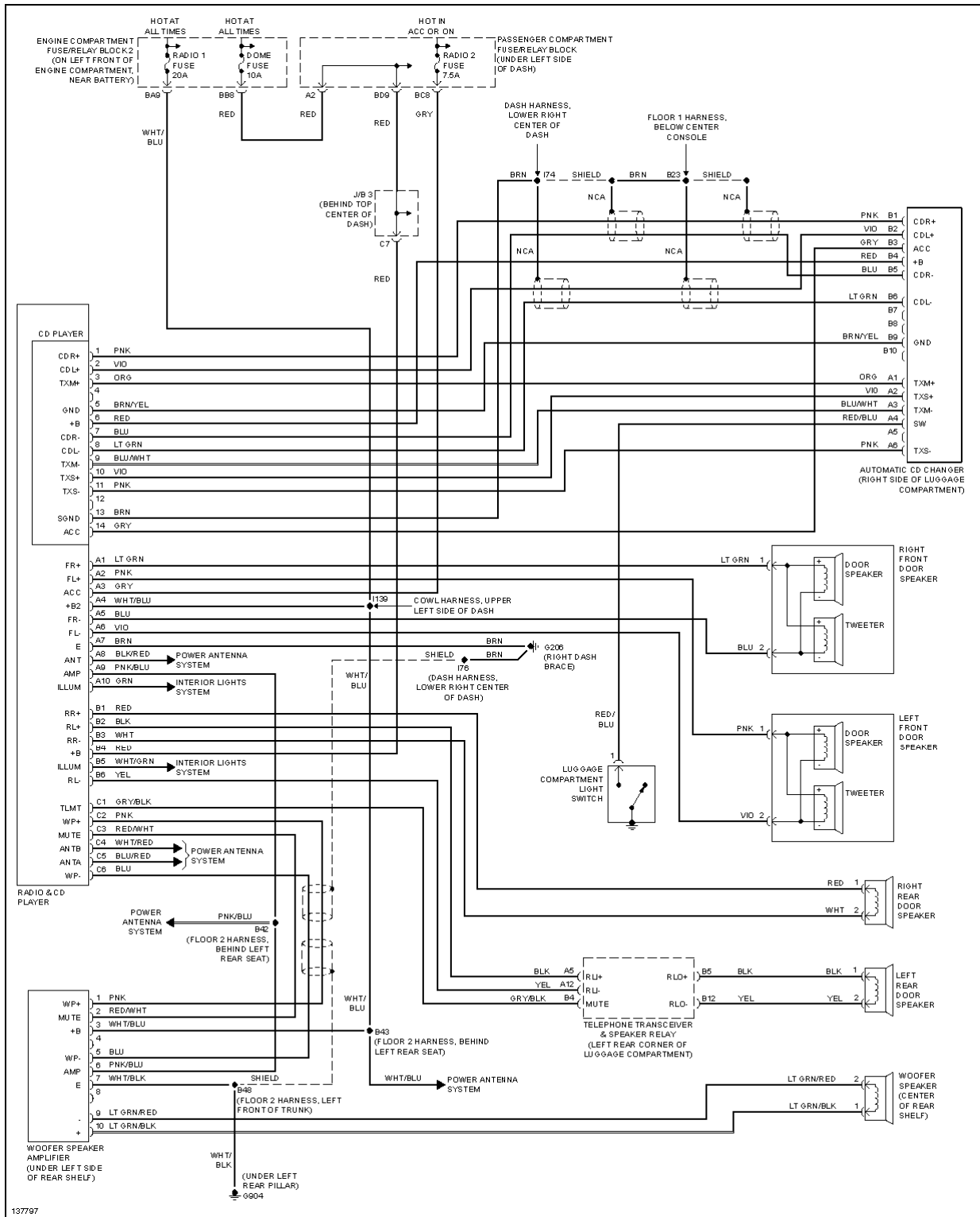
Fig. 53: Radio Circuits, Pioneer
