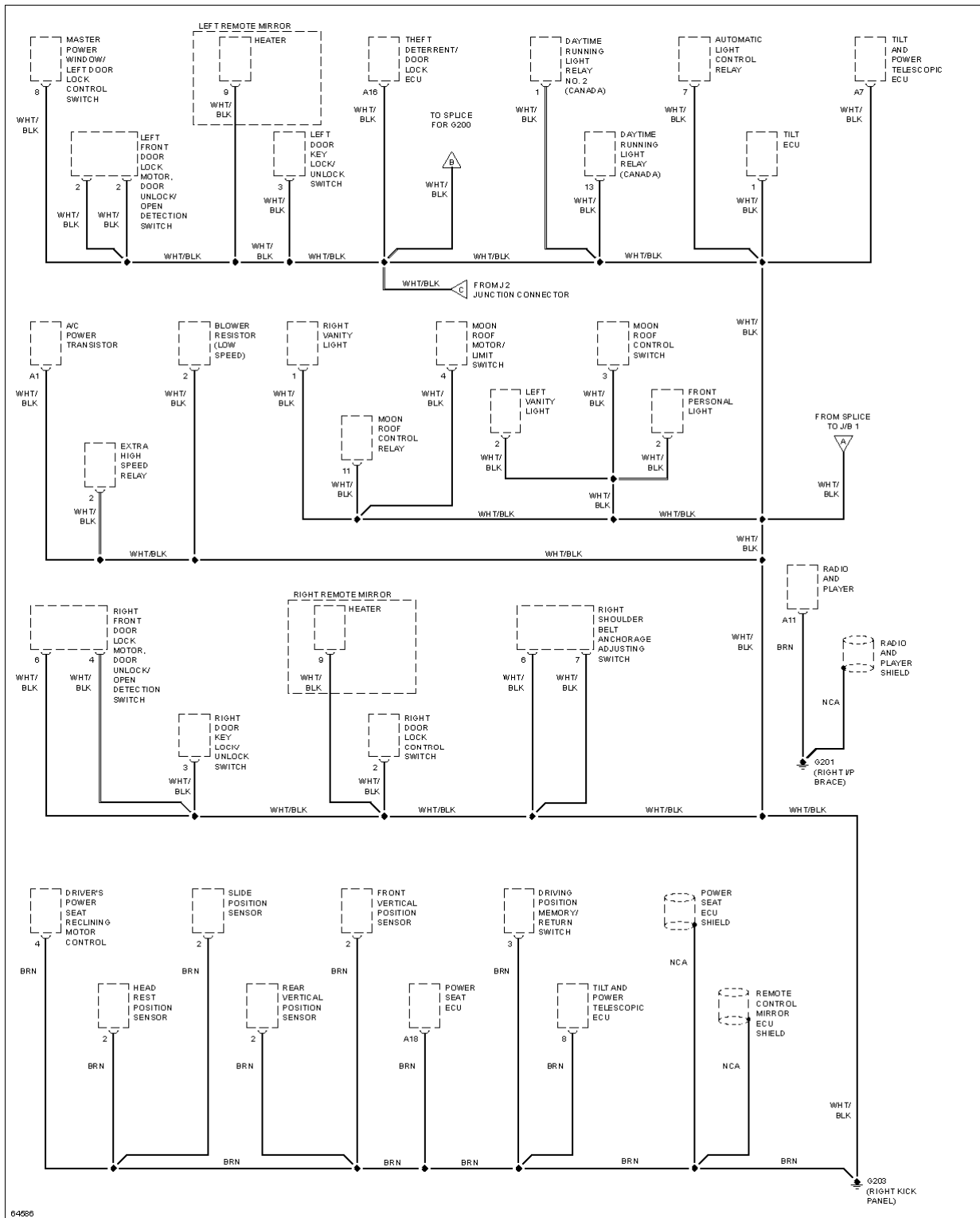
Fig. 23: Ground Distribution Circuit (3 of 5)
