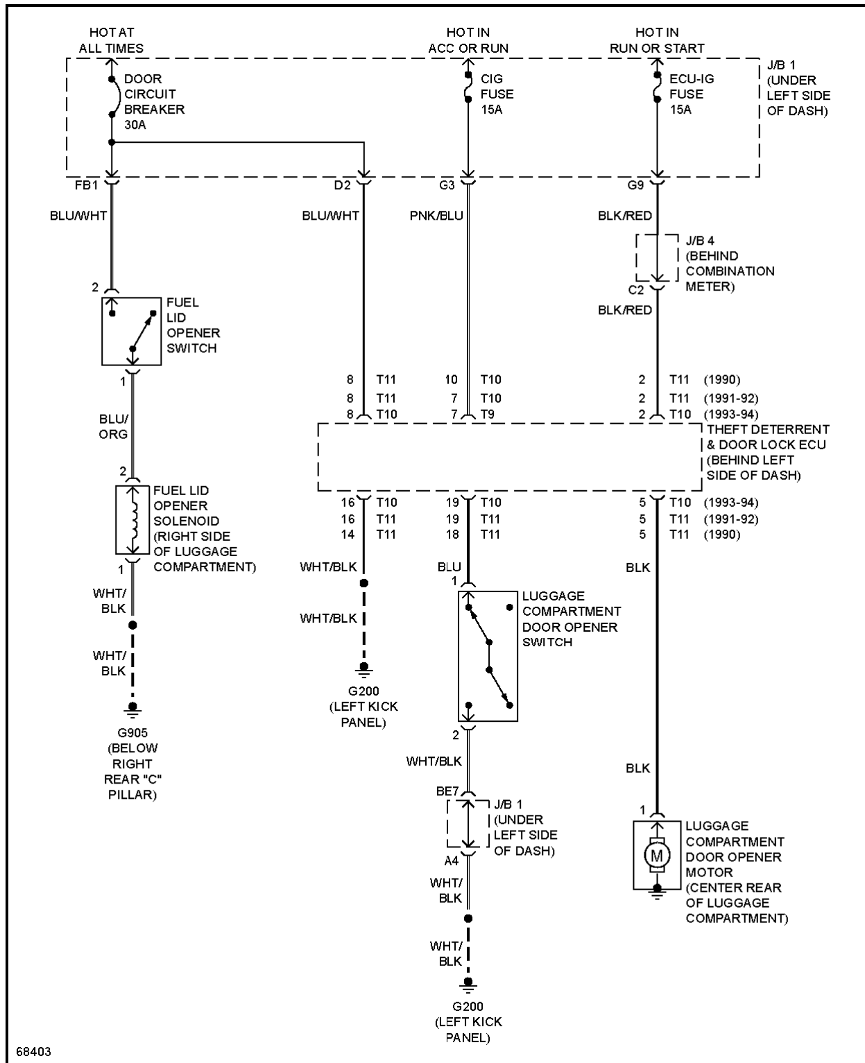
Fig. 59: Trunk & Fuel Door Release
