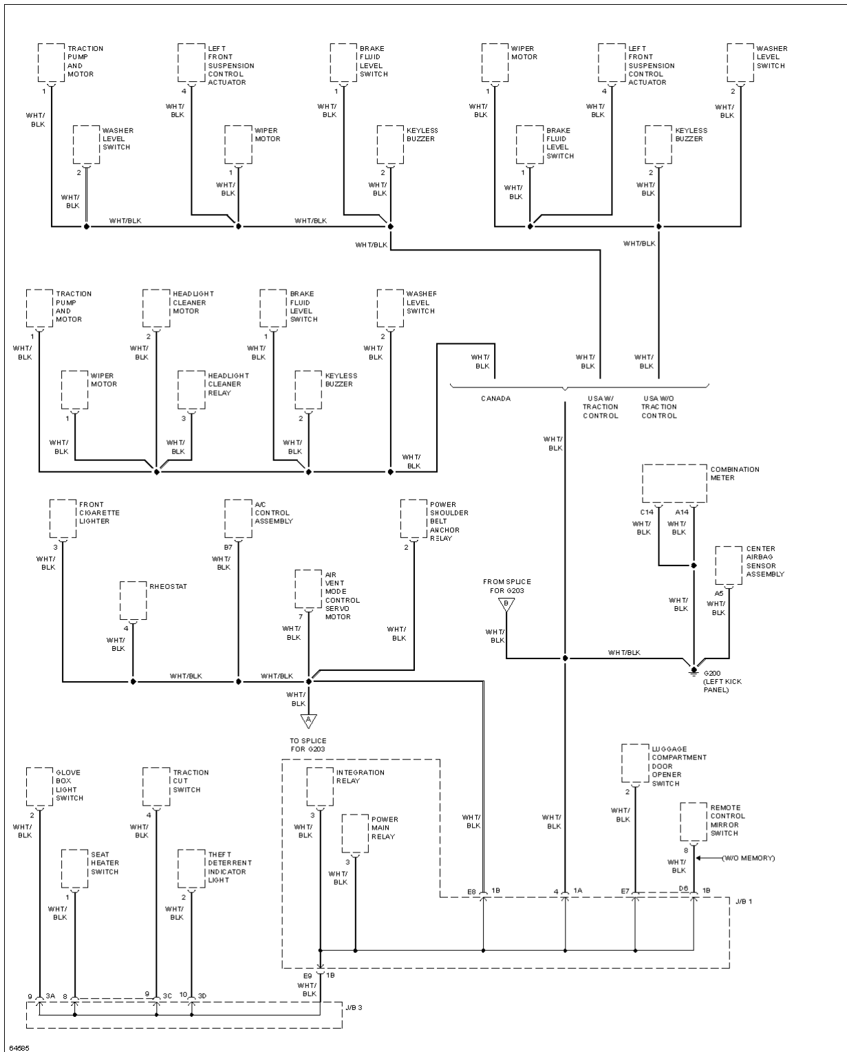
Fig. 22: Ground Distribution Circuit (2 of 5)
