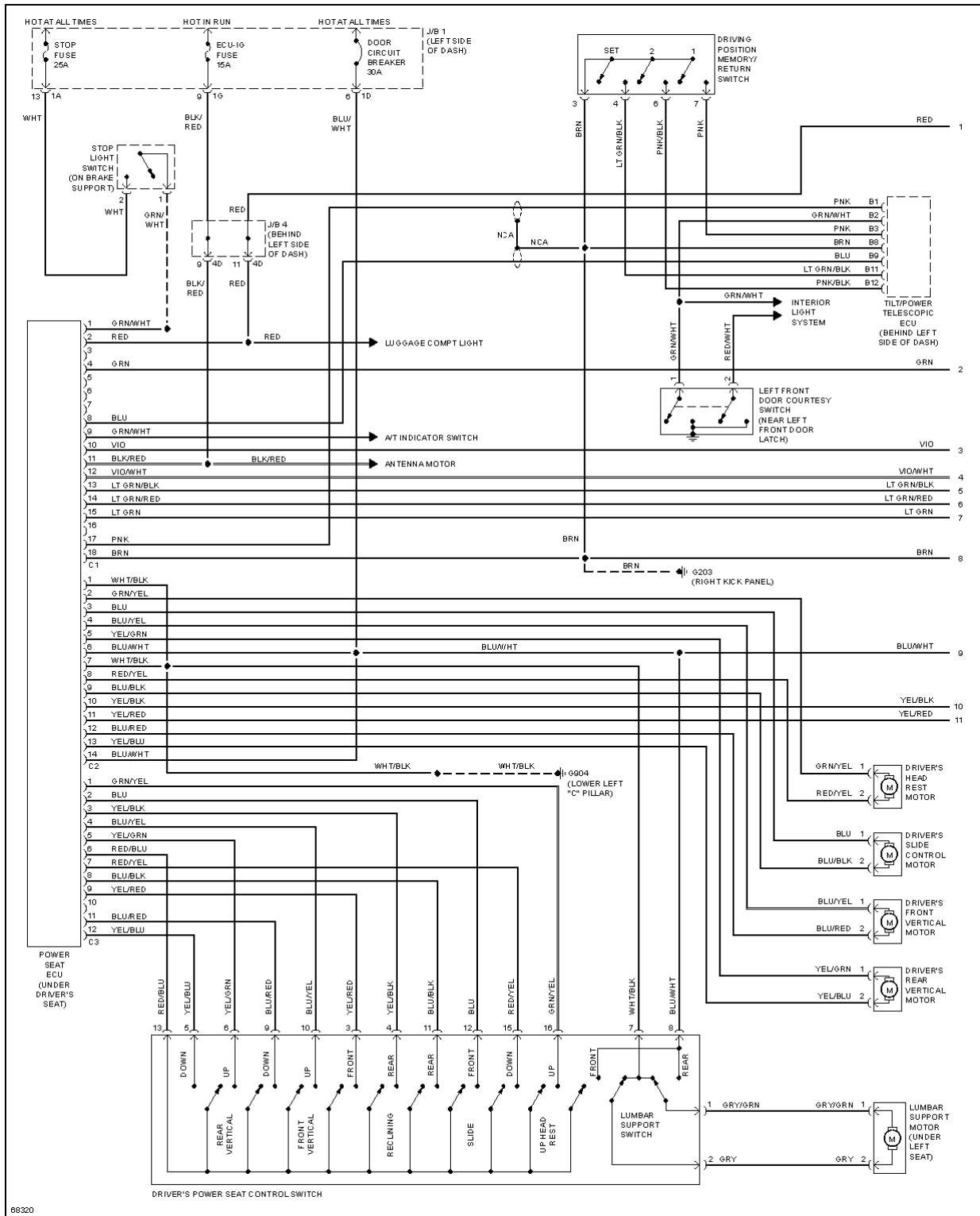
Fig. 35: Memory Seat Circuit (1 of 2)
