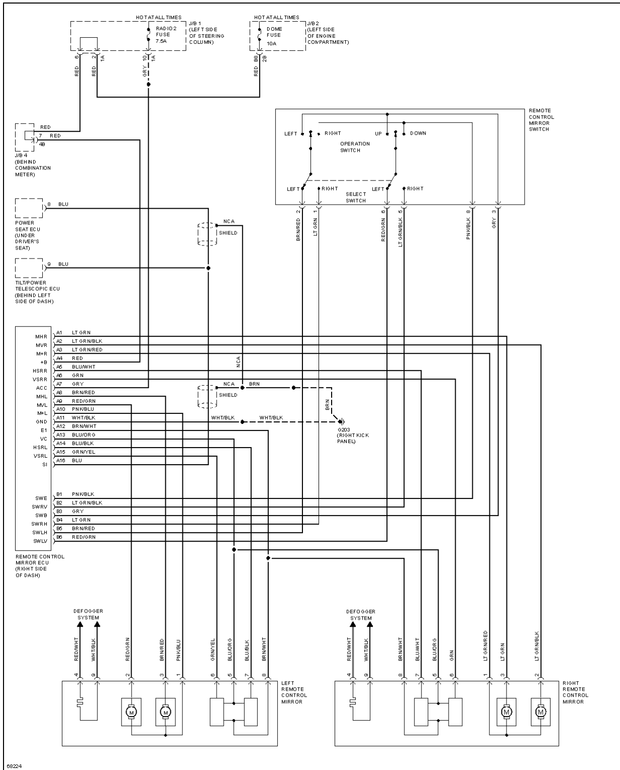
Fig. 33: Memory Mirrors Circuit
