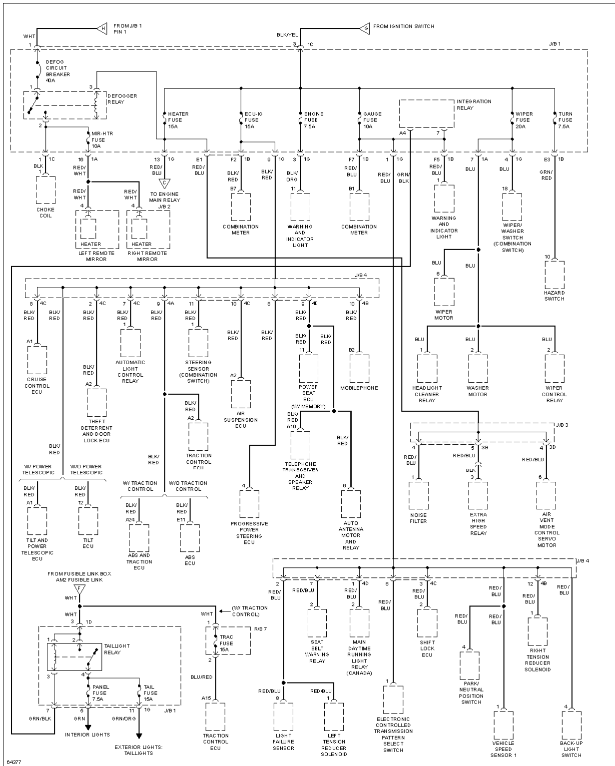
Fig. 42: Power Distribution Circuit (3 of 5)
