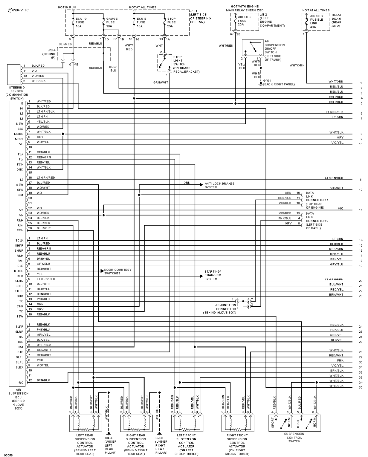
Fig. 14: Electronic Suspension Circuit (1 of 2)
