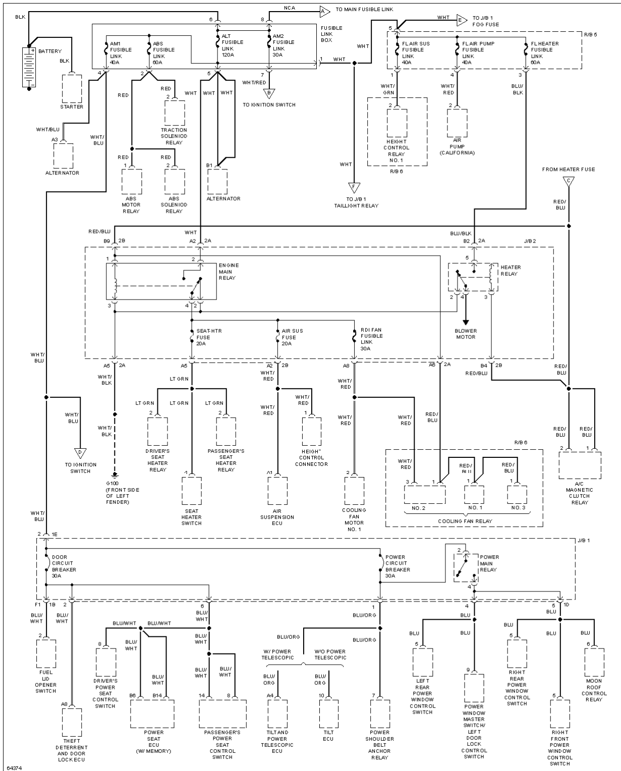
Fig. 40: Power Distribution Circuit (1 of 5)
