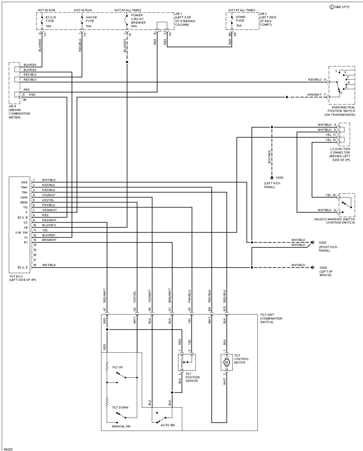
Fig. 13: Power Tilt Steering Column Circuit
