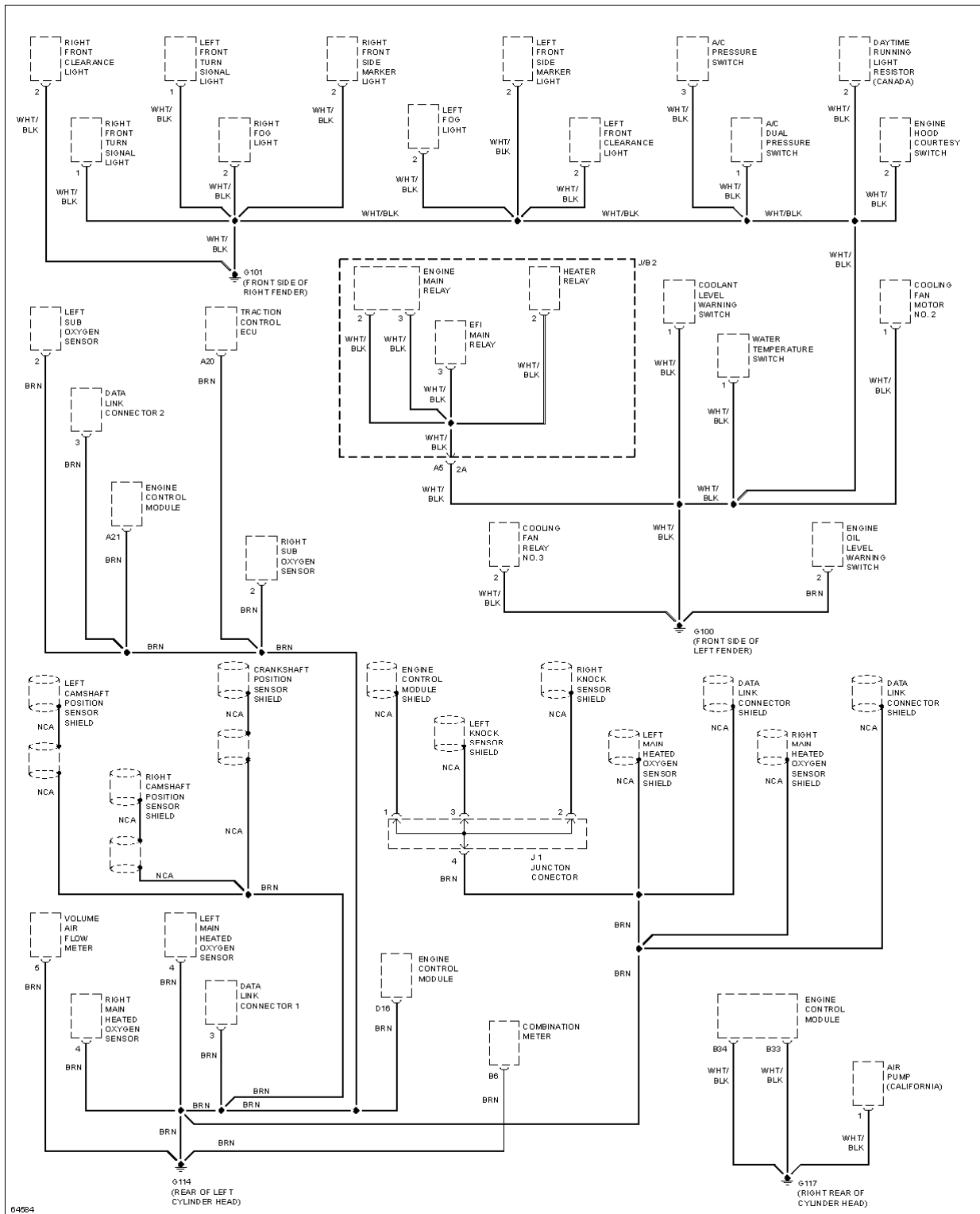
Fig. 21: Ground Distribution Circuit (1 of 5)
