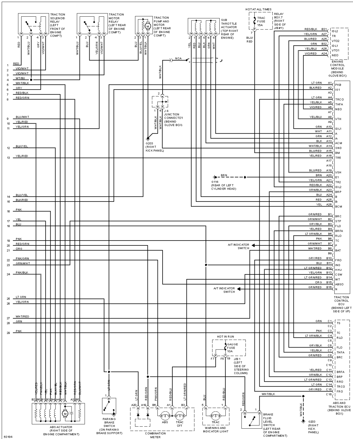
Fig. 6: Anti-lock Brake Circuits, W/ Traction Control (2 of 2)
