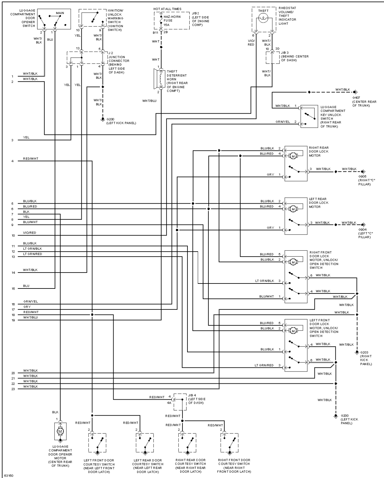
Fig. 46: Keyless Entry & Anti-Theft Circuit (2 of 2)
