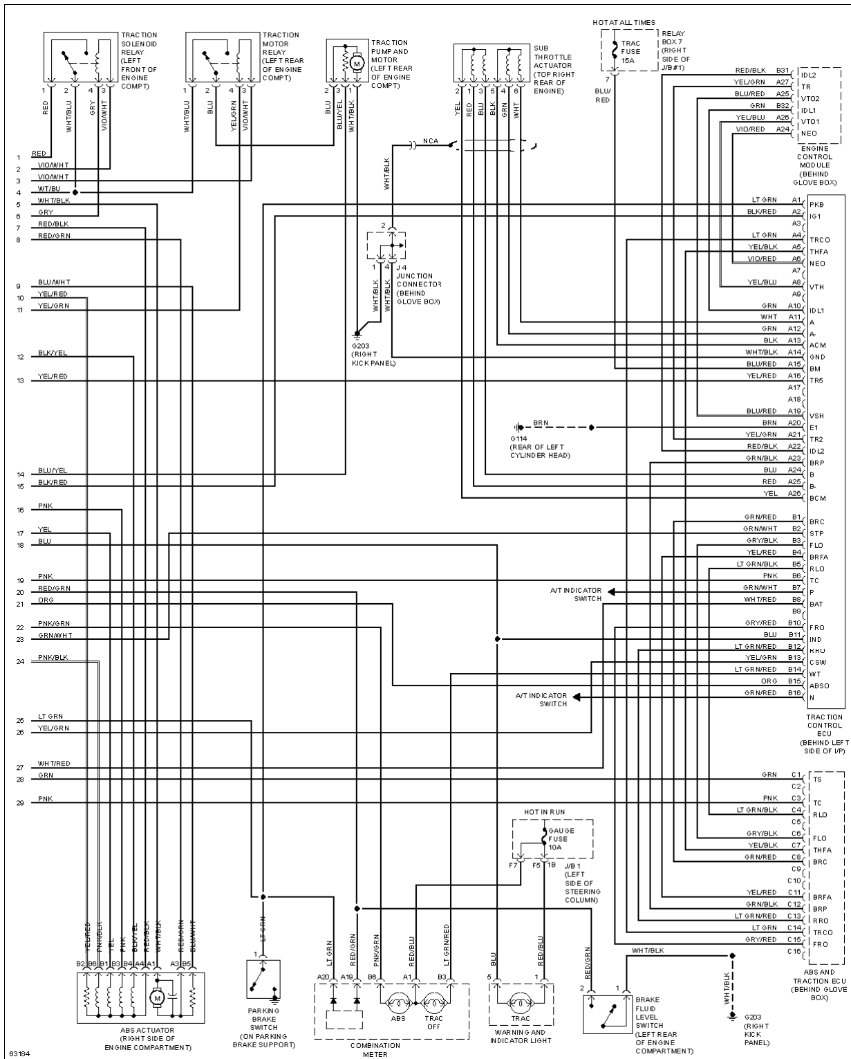
Fig. 5: Anti-lock Brake Circuits, W/ Traction Control (2 of 1)
