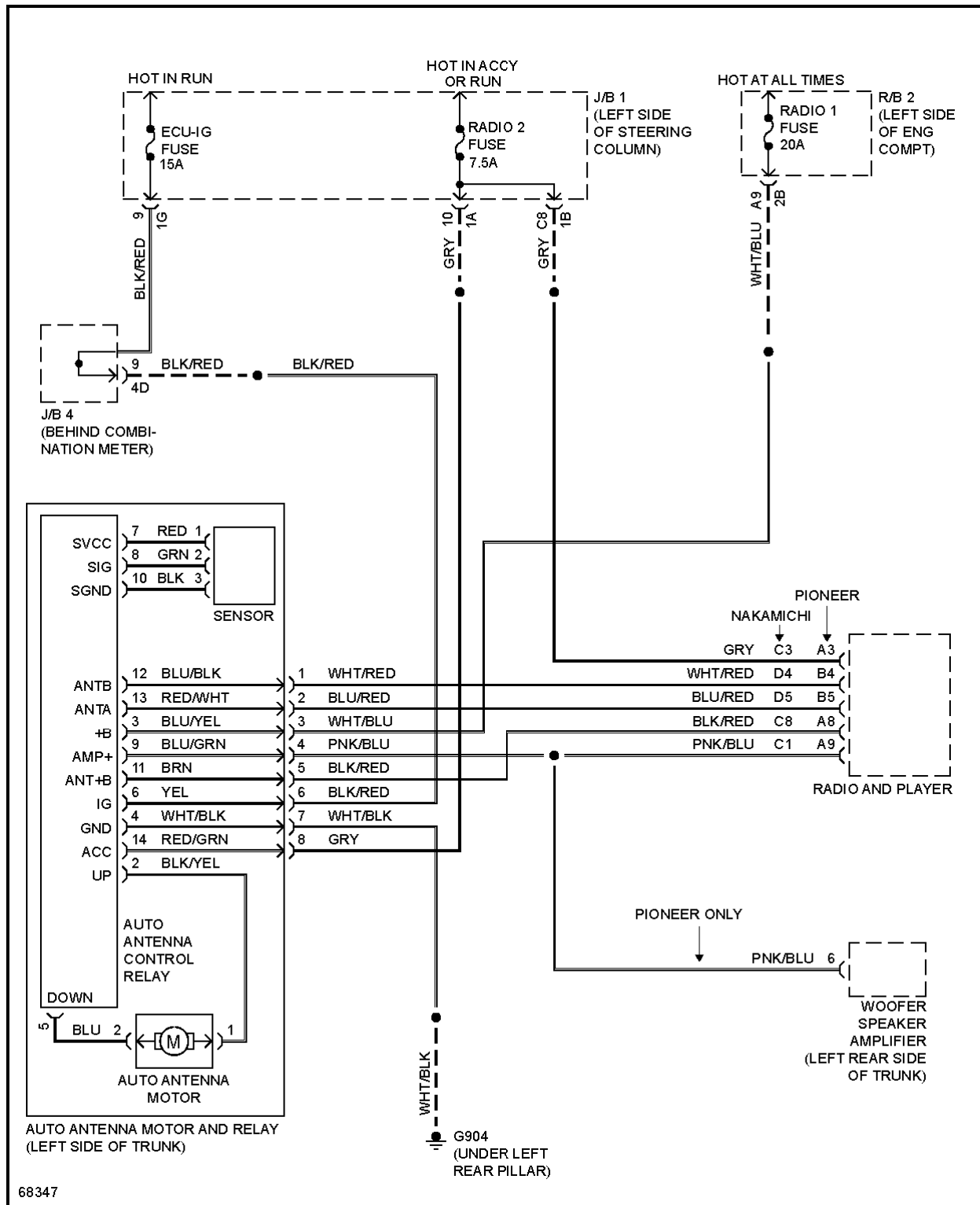
Fig. 39: Power Antenna Circuit
