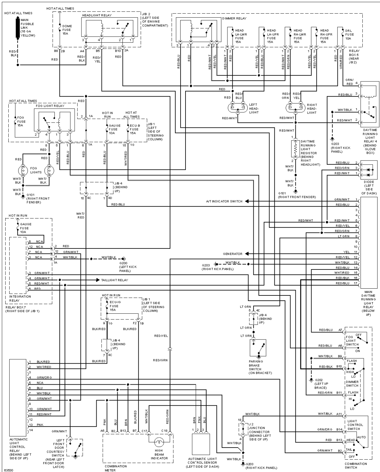
Fig. 26: Headlight Circuit, W/ DRL
