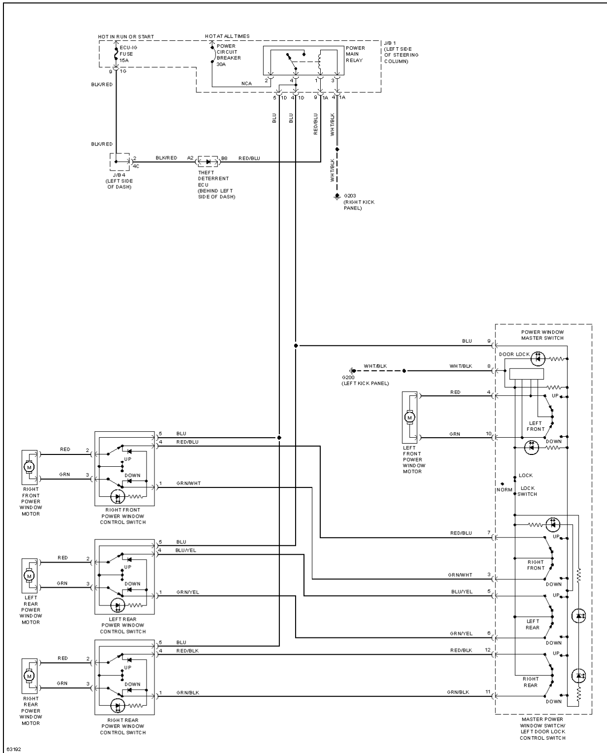
Fig. 51: Power Window Circuit
