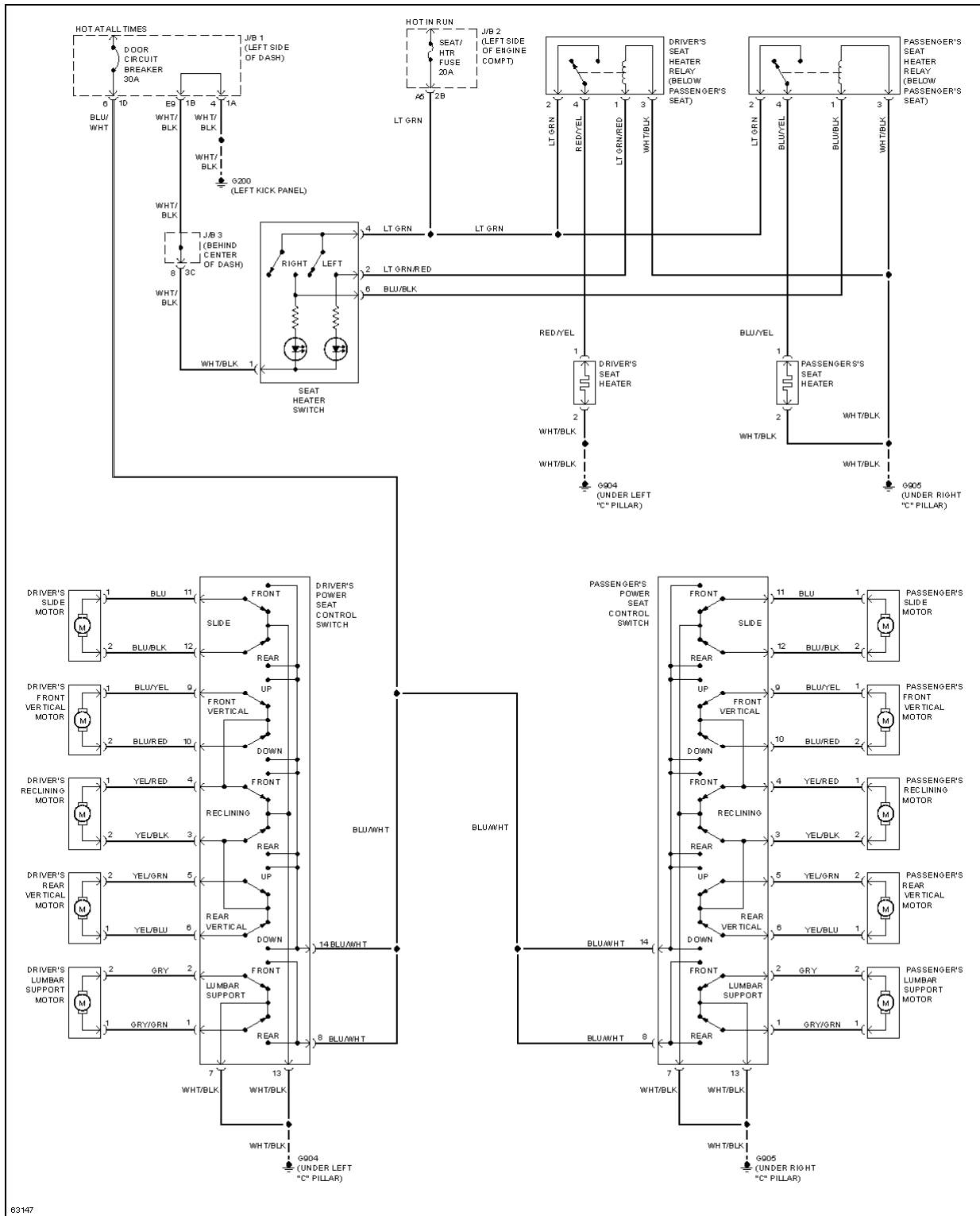
Fig. 49: Power Seat Circuits
