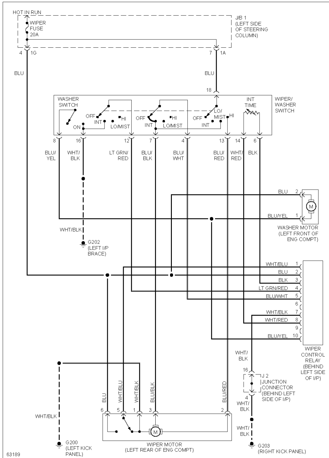
Fig. 61: Front Wiper/Washer Circuit
