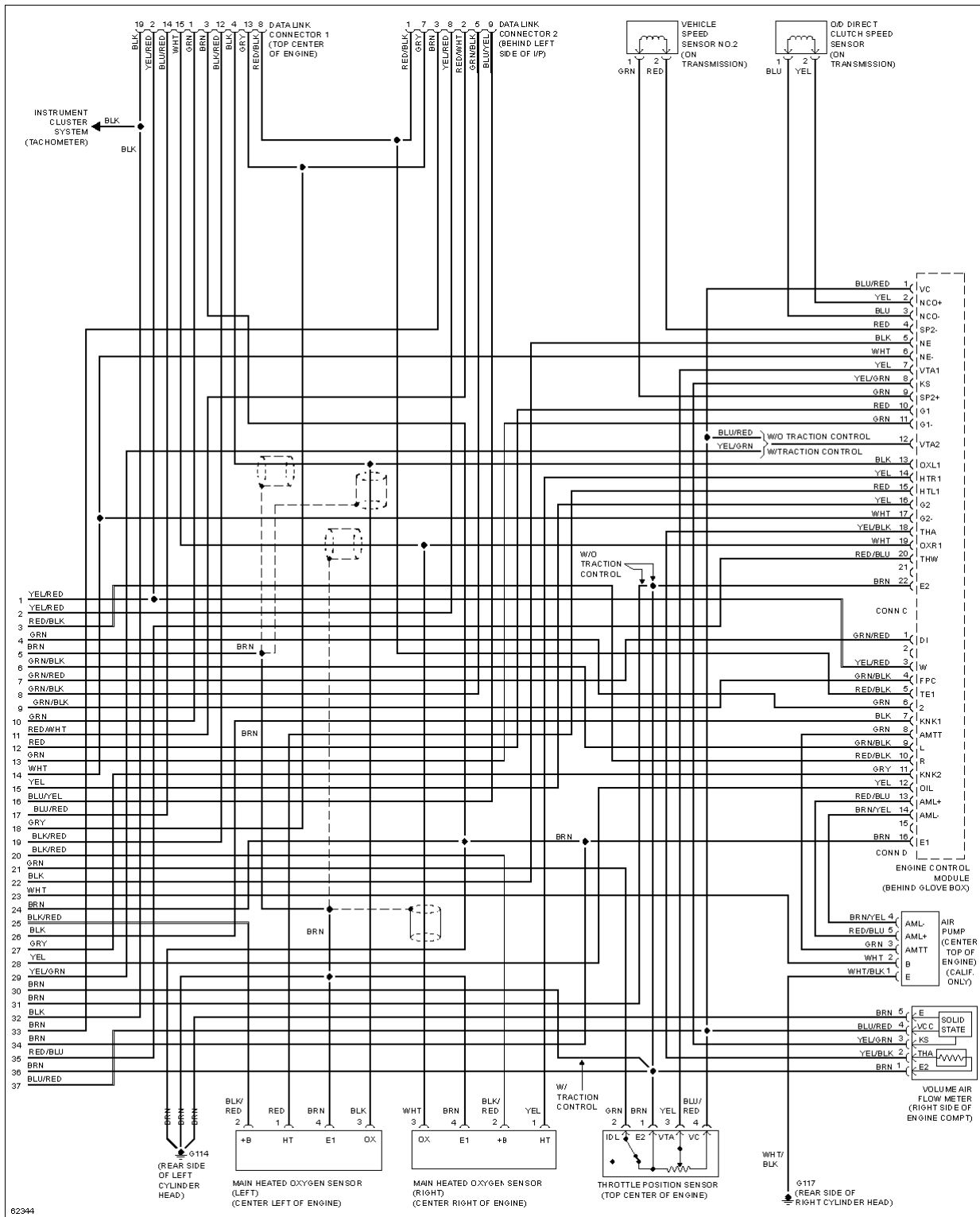
Fig. 18: 4.0L, Engine Performance Circuits (3 of 3)
