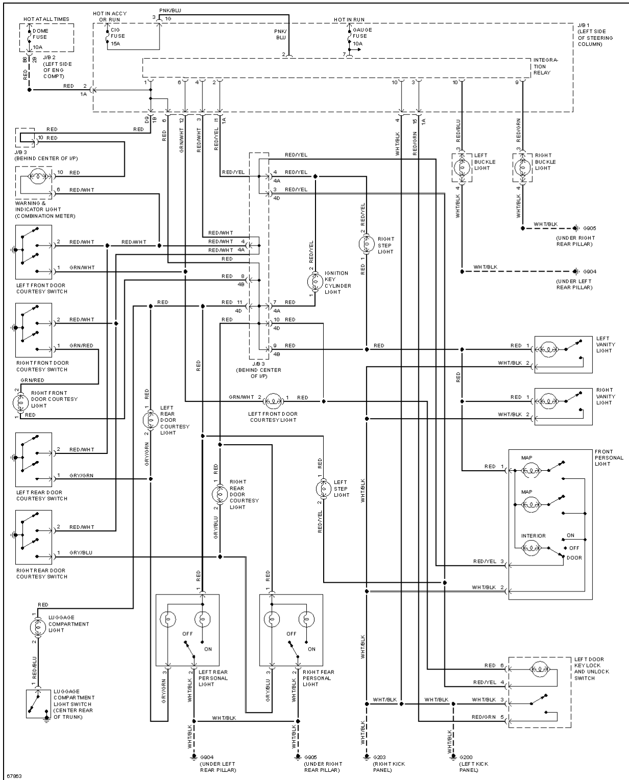
Fig. 31: Courtesy Lamp Circuit
