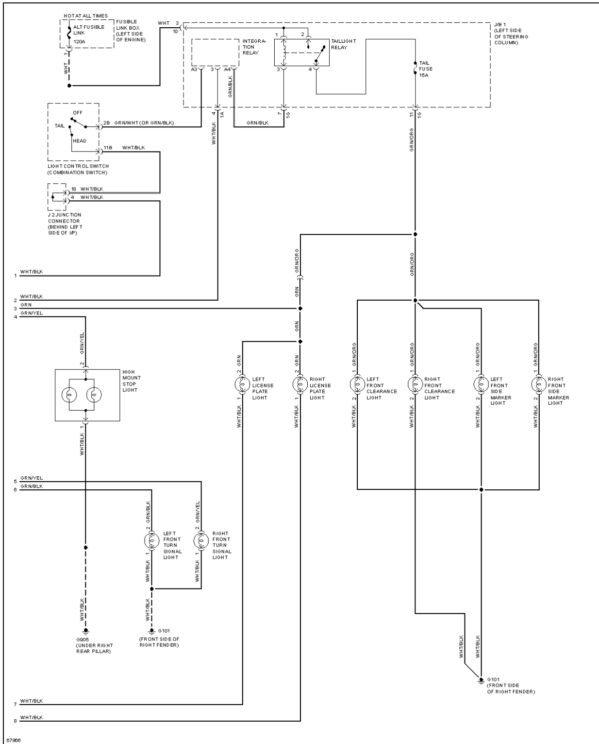
Fig. 20: Exterior Light Circuit (2 of 2)
