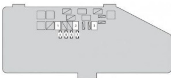
Scion iQ – fuse box – engine compartment (type
