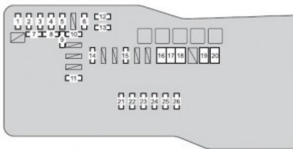
Scion iQ – fuse box – engine compartment (type
