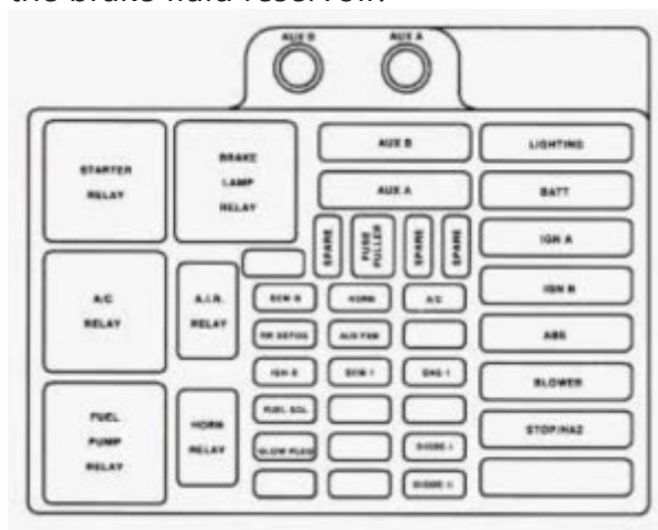
Chevrolet Suburban – fuse box – unerhood
