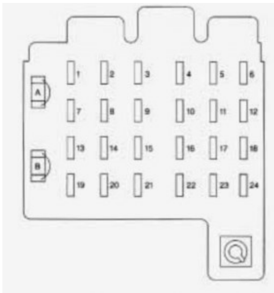
Chevrolet Suburban – fuse box – instrument panel
