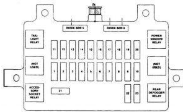
Isuzu Rodeo – fuse box diagram
