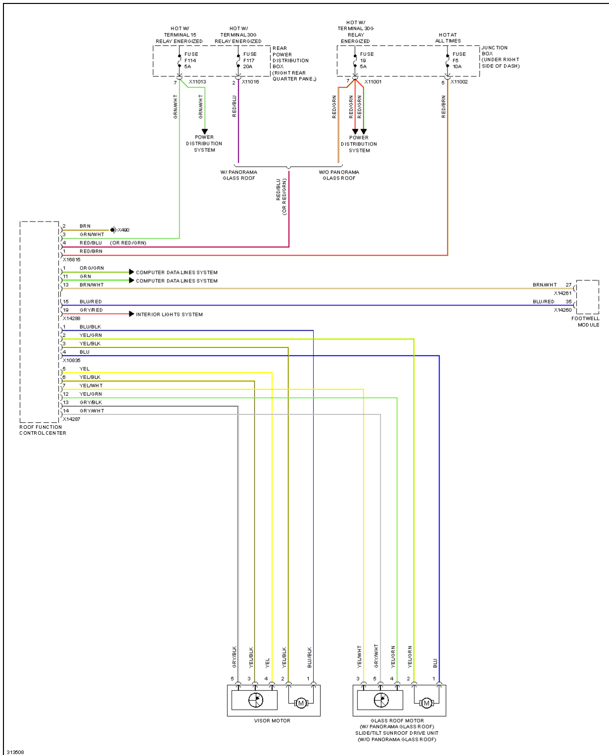
Fig. 101: Power Top/Sunroof Circuit
