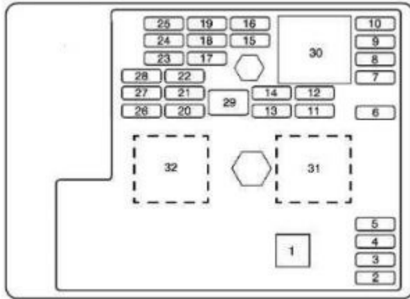
Chevrolet HHR – fuse box diagram – passenger
