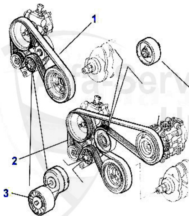
Keilrippenriemen V-BELTS 145/6 TS 16V
