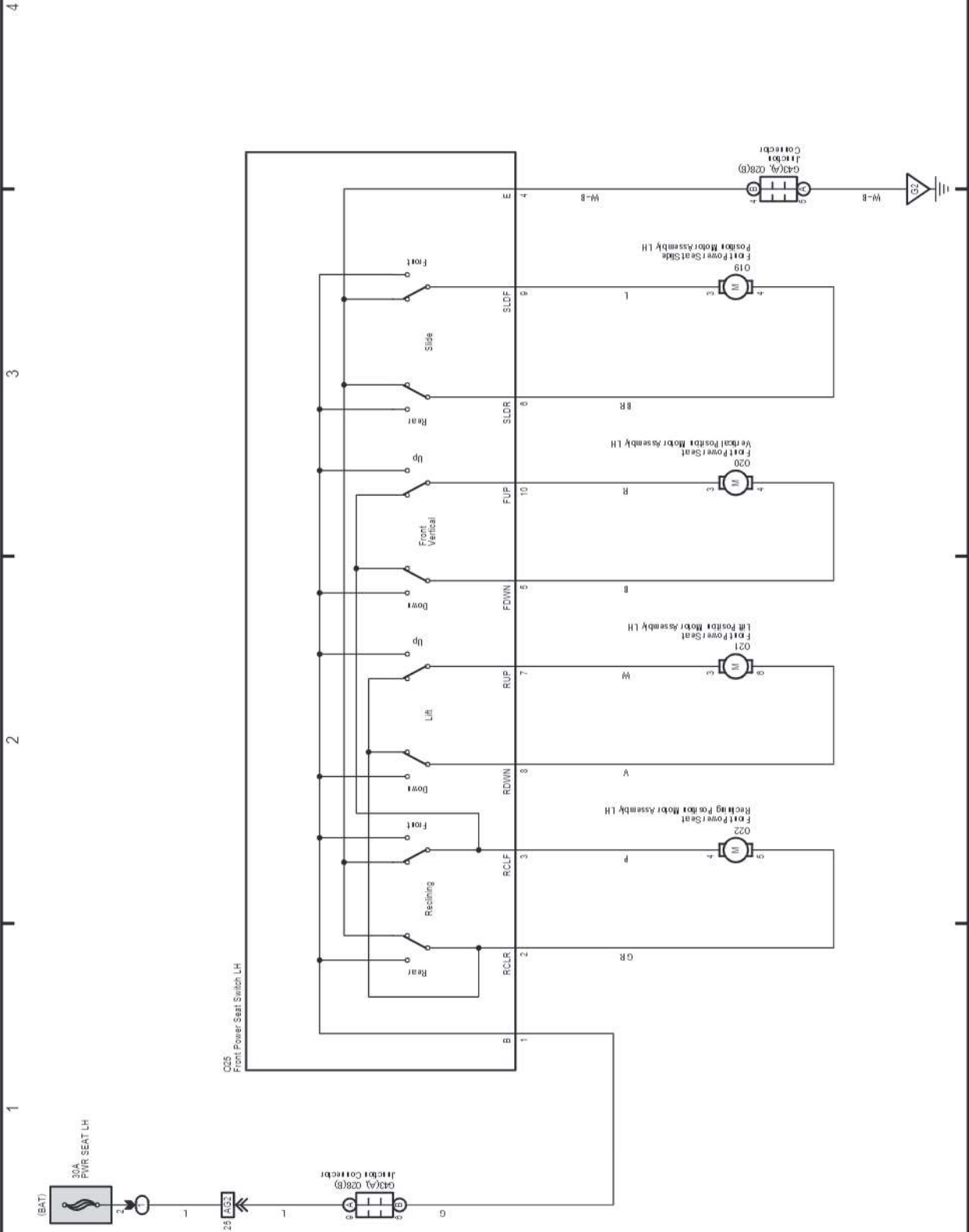
Power Seat (RHD Front Passenger's Seat)
