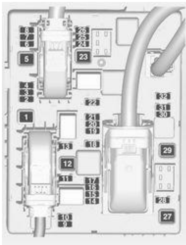
Vauxhall Zafira C Tourer – fuse box – load compartment
