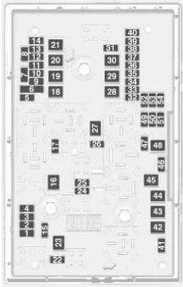
Vauxhall Zafira C Tourer – fuse box – engine
