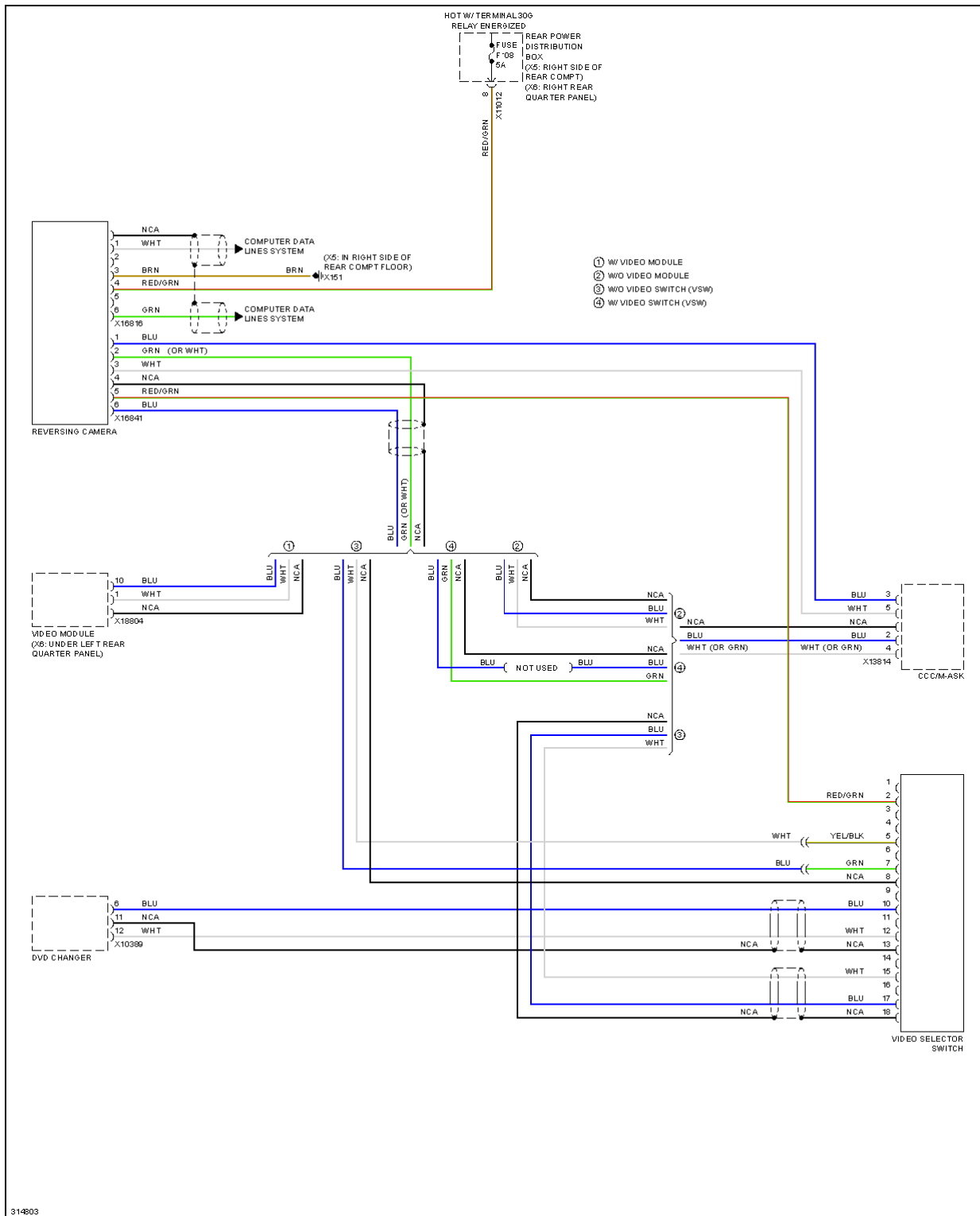
Fig. 80: Rear Camera Circuit
