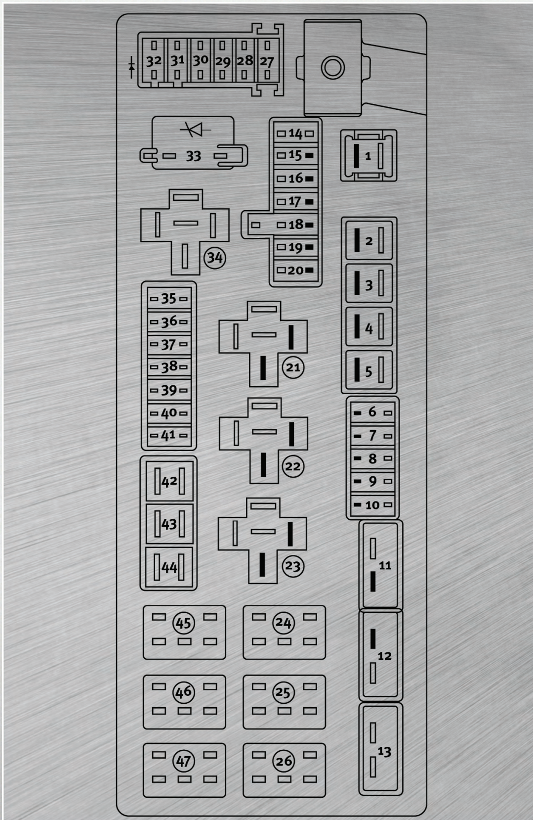
Fuses – Rear Power Distribution Center
