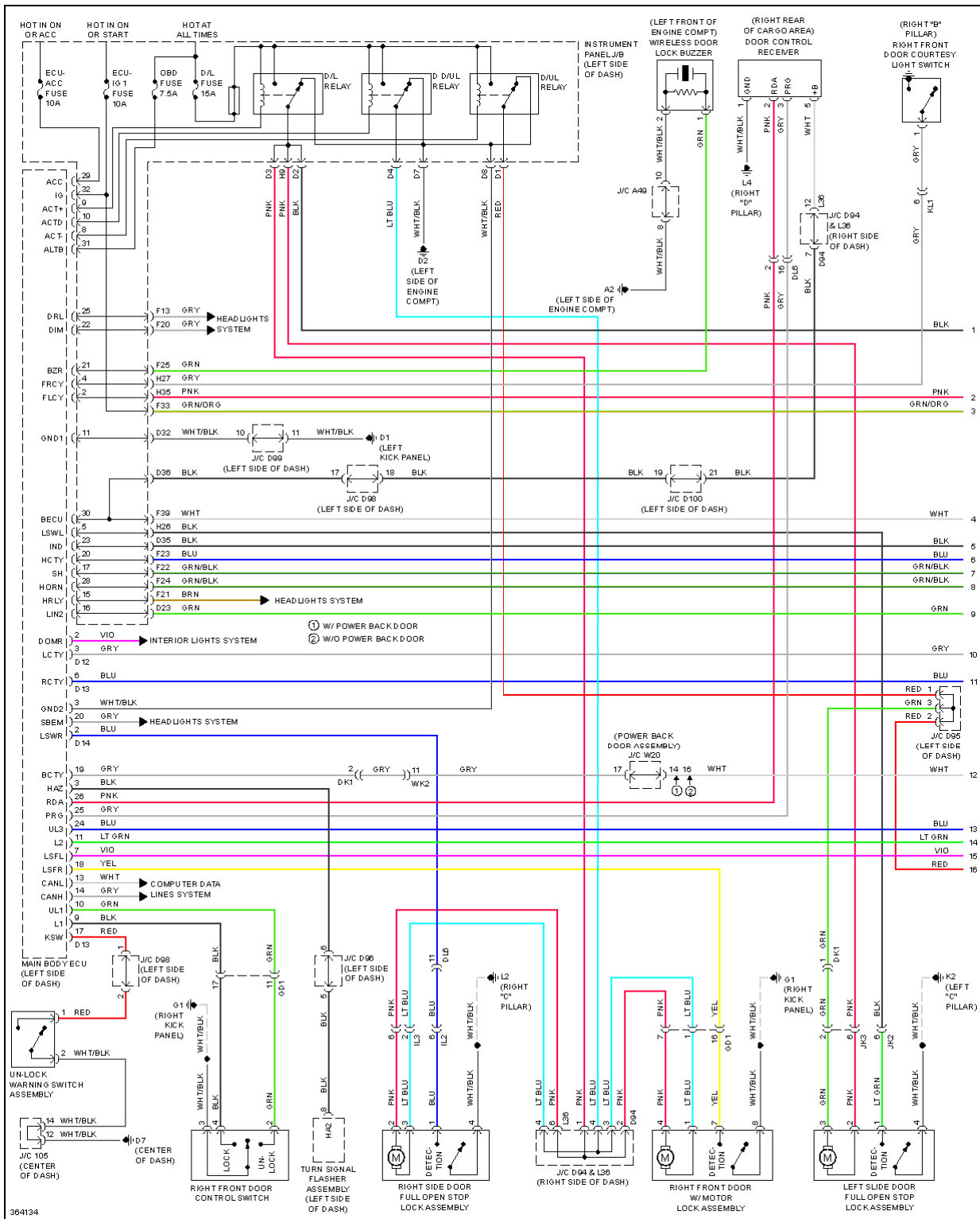
Fig. 78: Power Door Locks Circuit, W/O Smart Key System (1 of 2)
