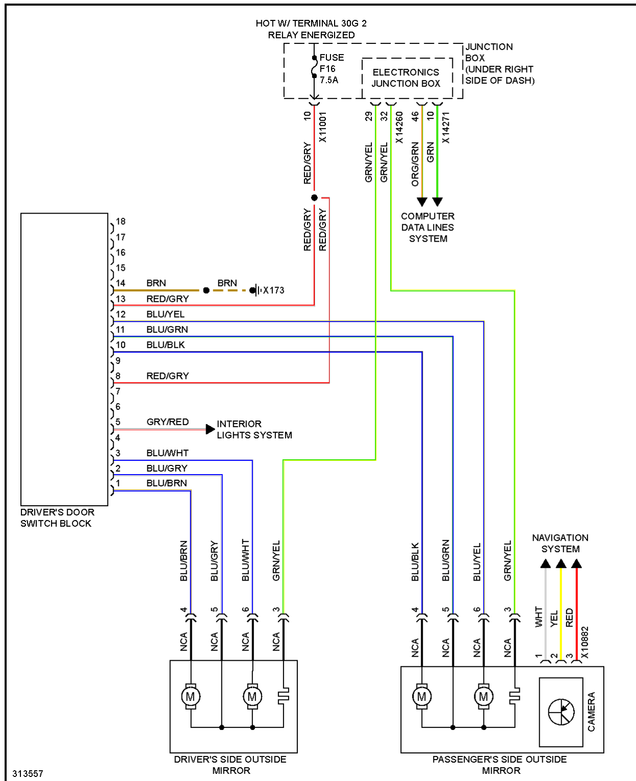
Fig. 65: Power Mirrors Circuit, W/O LIN bus Function
