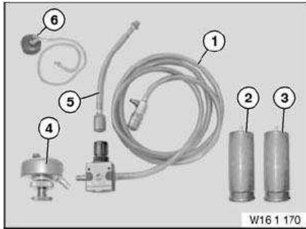
Fig. 3: Identifying Special Tool (16 1 170) Courtesy of BMW OF NORTH AMERICA, INC.
