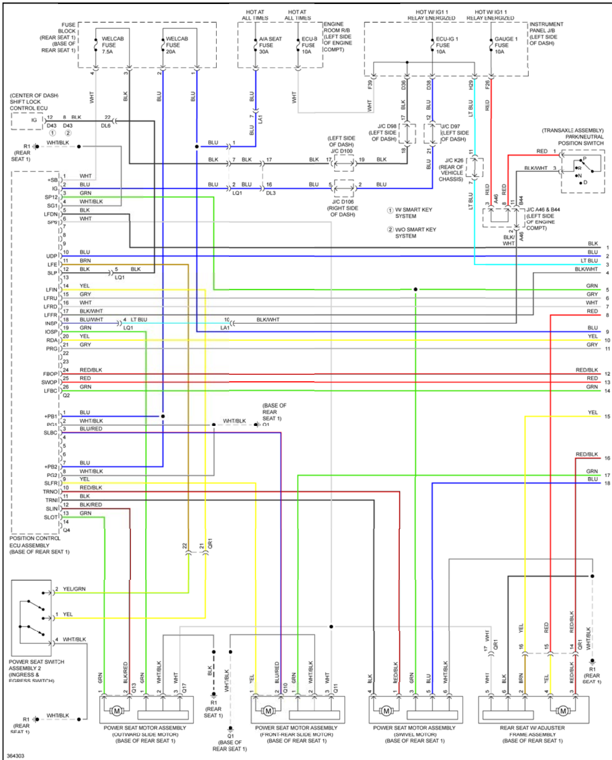
Fig. 82: Auto Access Seat Circuit (1 of 2)
