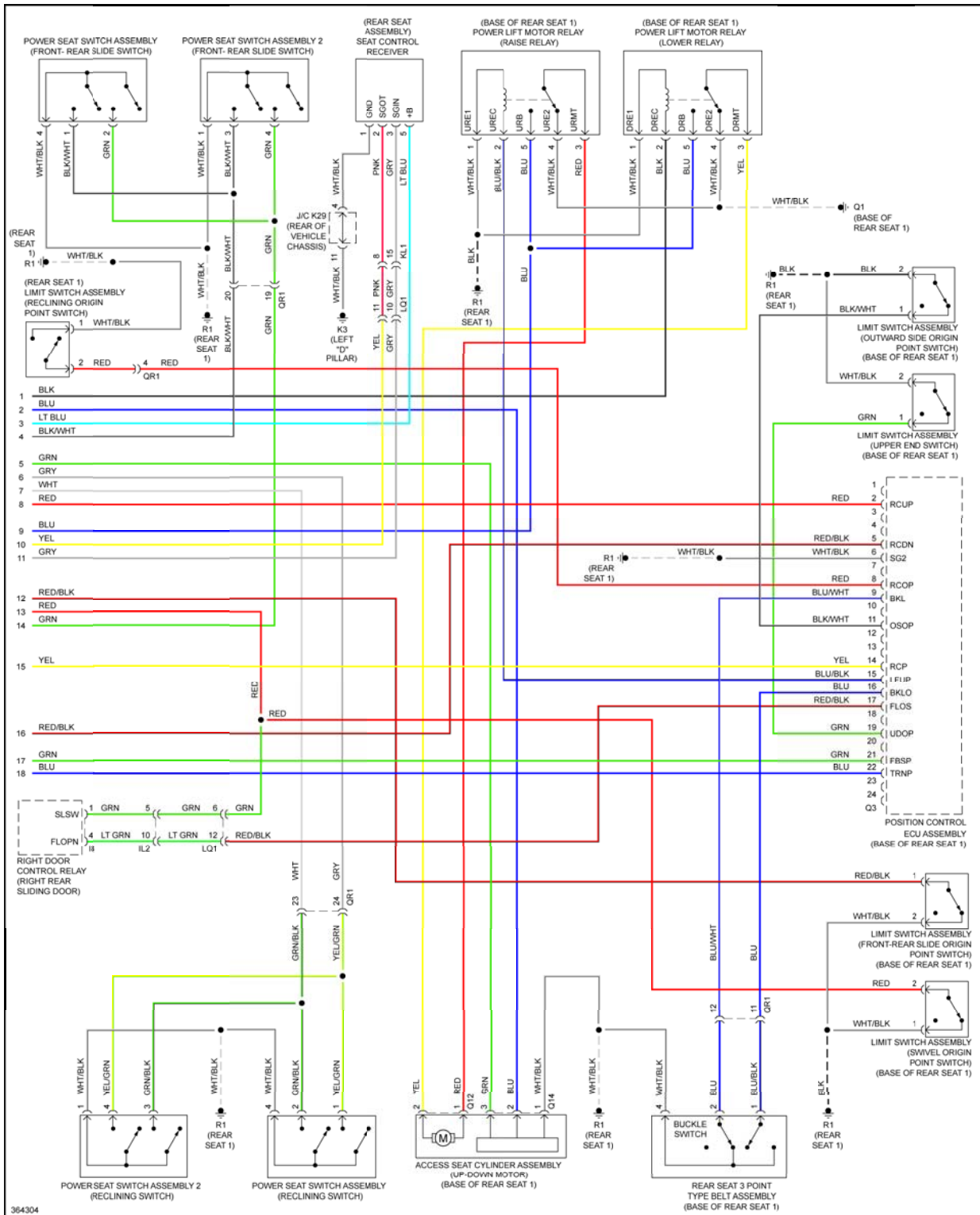
Fig. 83: Auto Access Seat Circuit (2 of 2)
