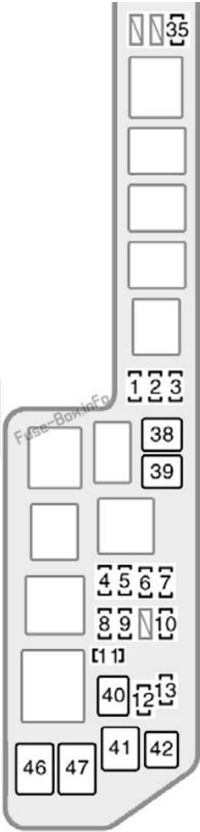
Engine Compartment Fuse Box #1
