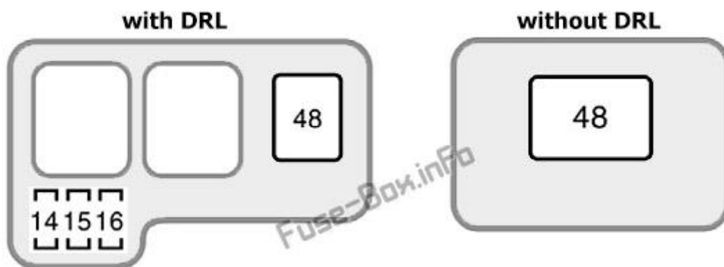
Assignment of the fuses in the Fuse Box #2 (1998-2000)
