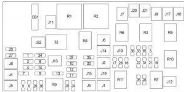
Dodge Ram 1500 – fuse box diagram
