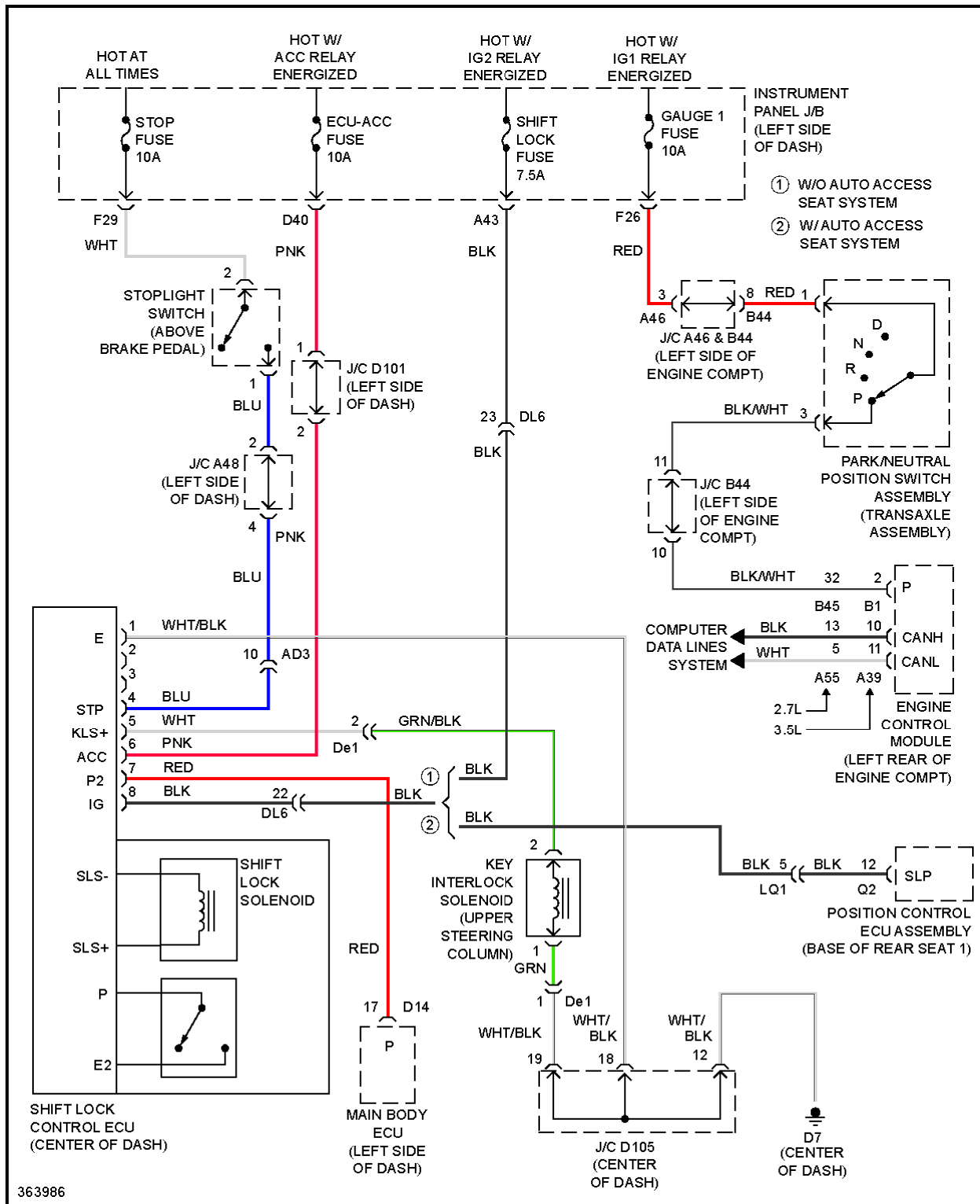
Fig. 103: Shift Interlock Circuit, W/O Smart Key System
