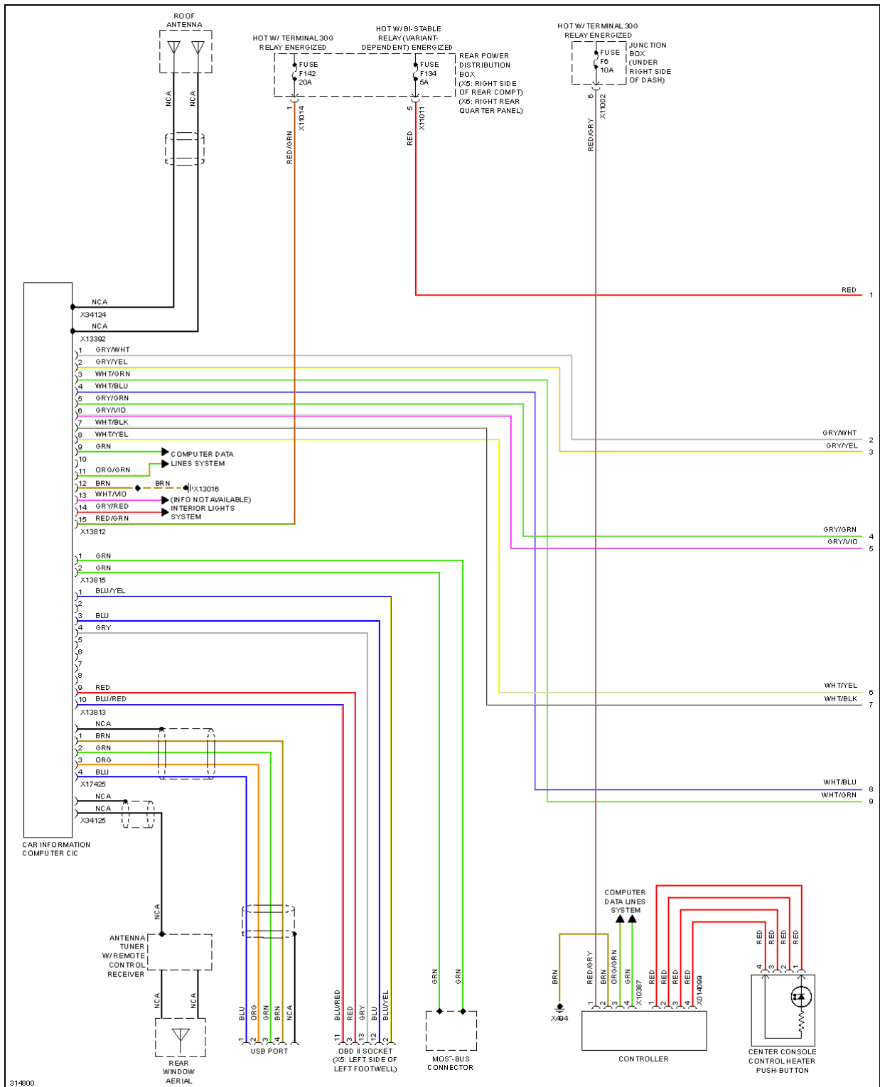
Fig. 70: Navigation Circuit, W/ CIC & HIFI Radio (1 of 2)
