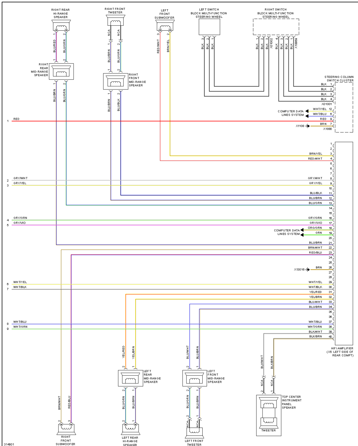
Fig. 71: Navigation Circuit, W/ CIC & HIFI Radio (2 of 2)
