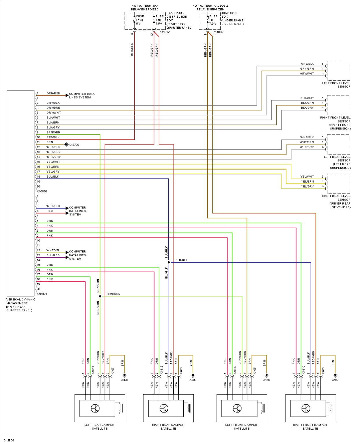
Fig. 31: Electronic Damper Control Circuit
