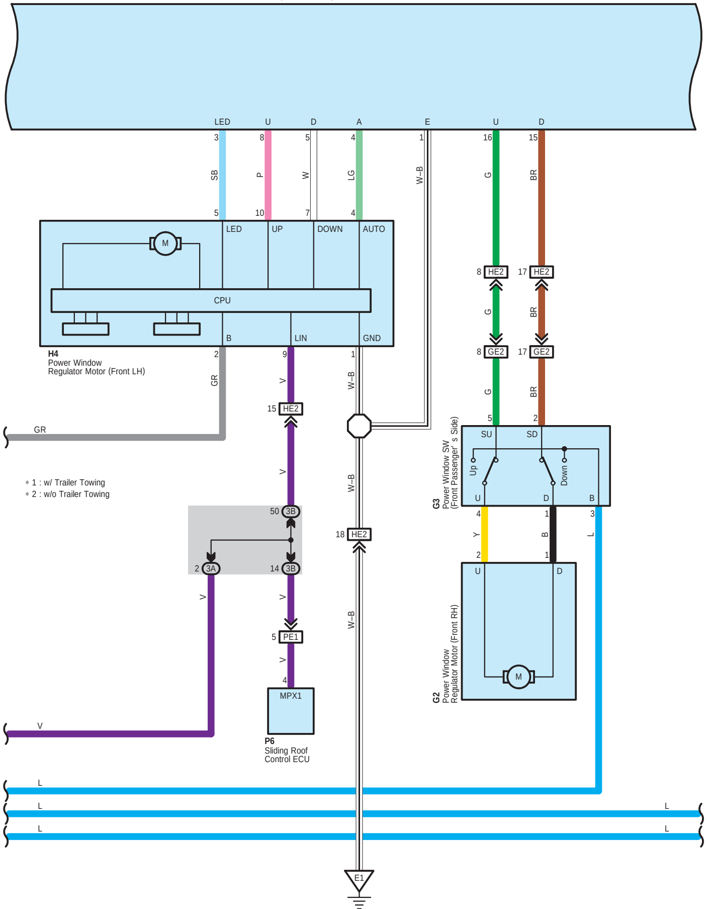
H2 Power Window SW (Driver' s Side)
