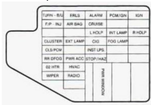
Chevrolet Cavalier – fuse box – instrument panel
