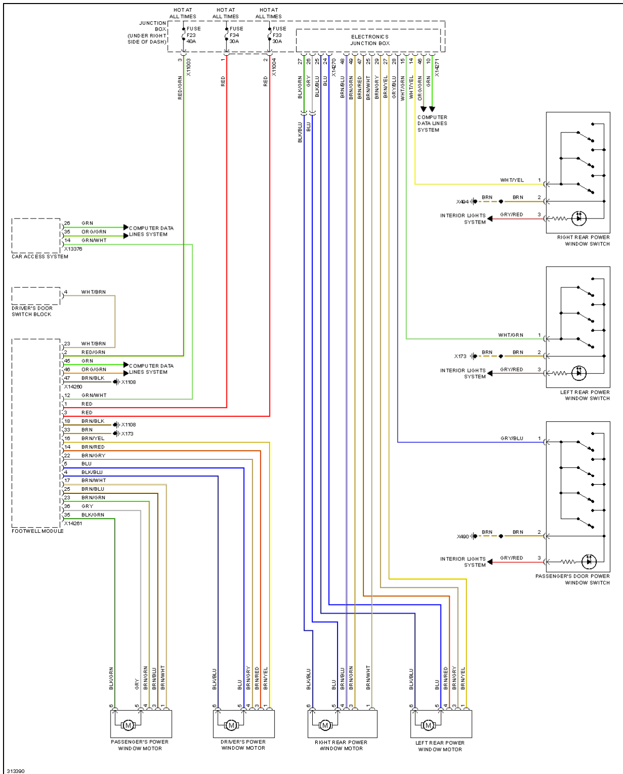
Fig. 102: Power Windows Circuit
