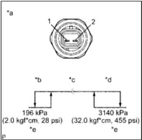
(a) Connect a manifold gauge set.
