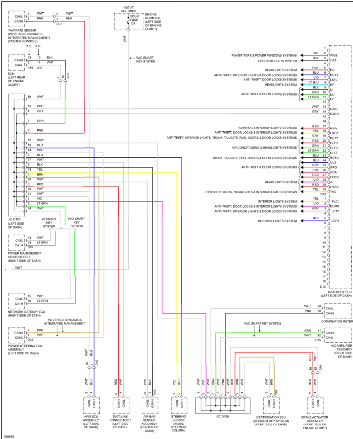
Fig. 14: Body ECU Circuit (2 of 2)
