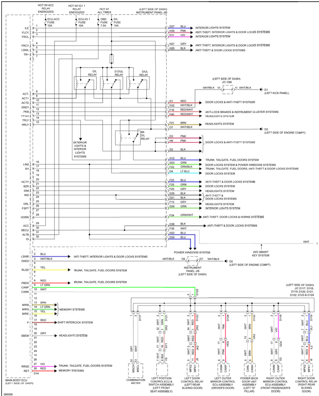
Fig. 13: Body ECU Circuit (1 of 2)
