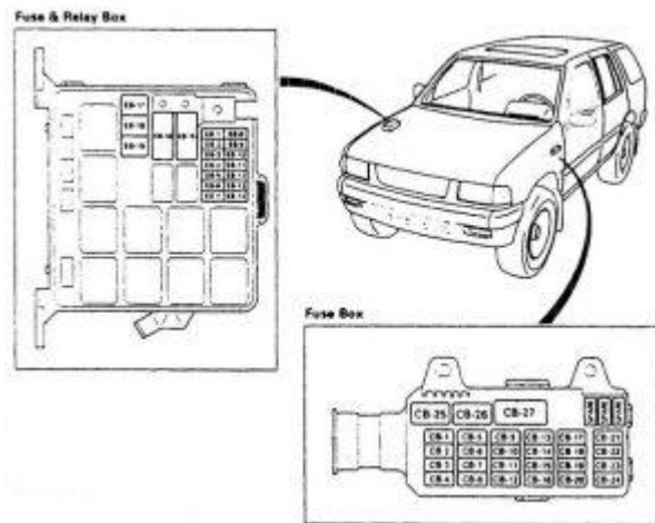
Isuzu Rodeo – fuse box diagram
