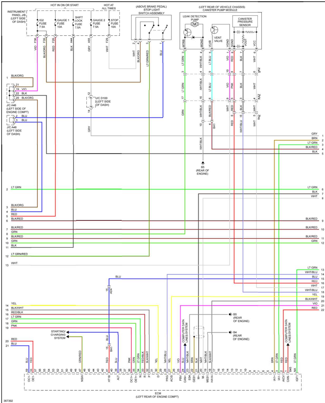
Fig. 30: 2.7L, Engine Performance Circuit (2 of 4)
