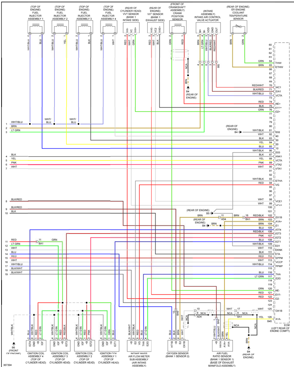
Fig. 32: 2.7L, Engine Performance Circuit (4 of 4)
