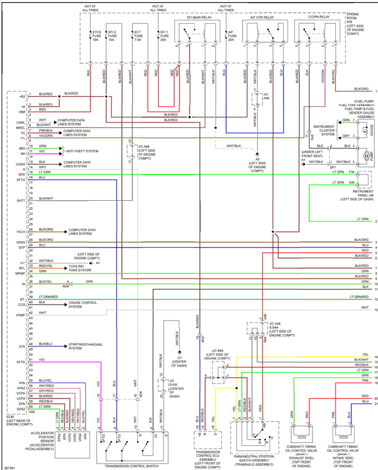
Fig. 29: 2.7L, Engine Performance Circuit (1 of 4)
