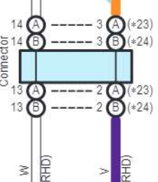
E77(A), E115(B) Junction Connector
