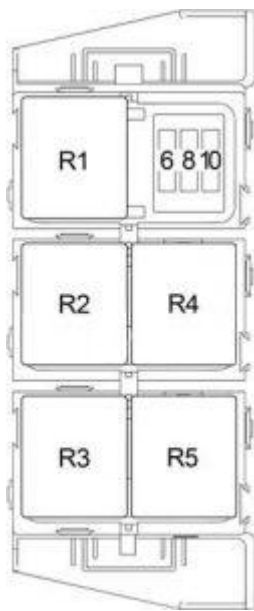
Dodge Caliber – fuse box diagram
