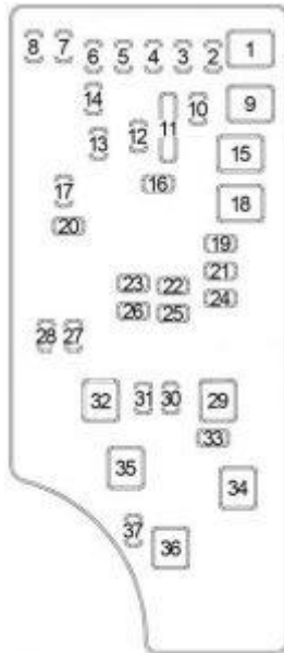
Dodge Caliber – fuse box diagram
