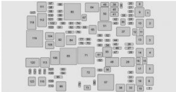
GMC Yukon – fuse box – engine compartment
