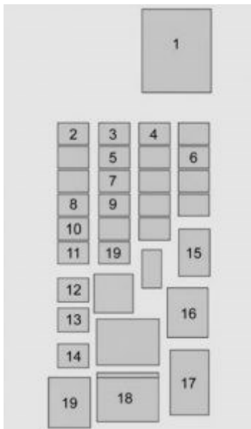
GMC Yukon – fuse box – rear compartment
