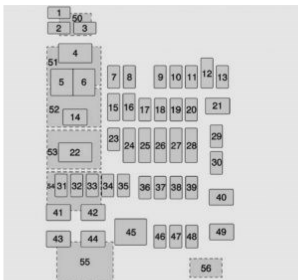
GMC Yukon – fuse box – instrument panel (left)
