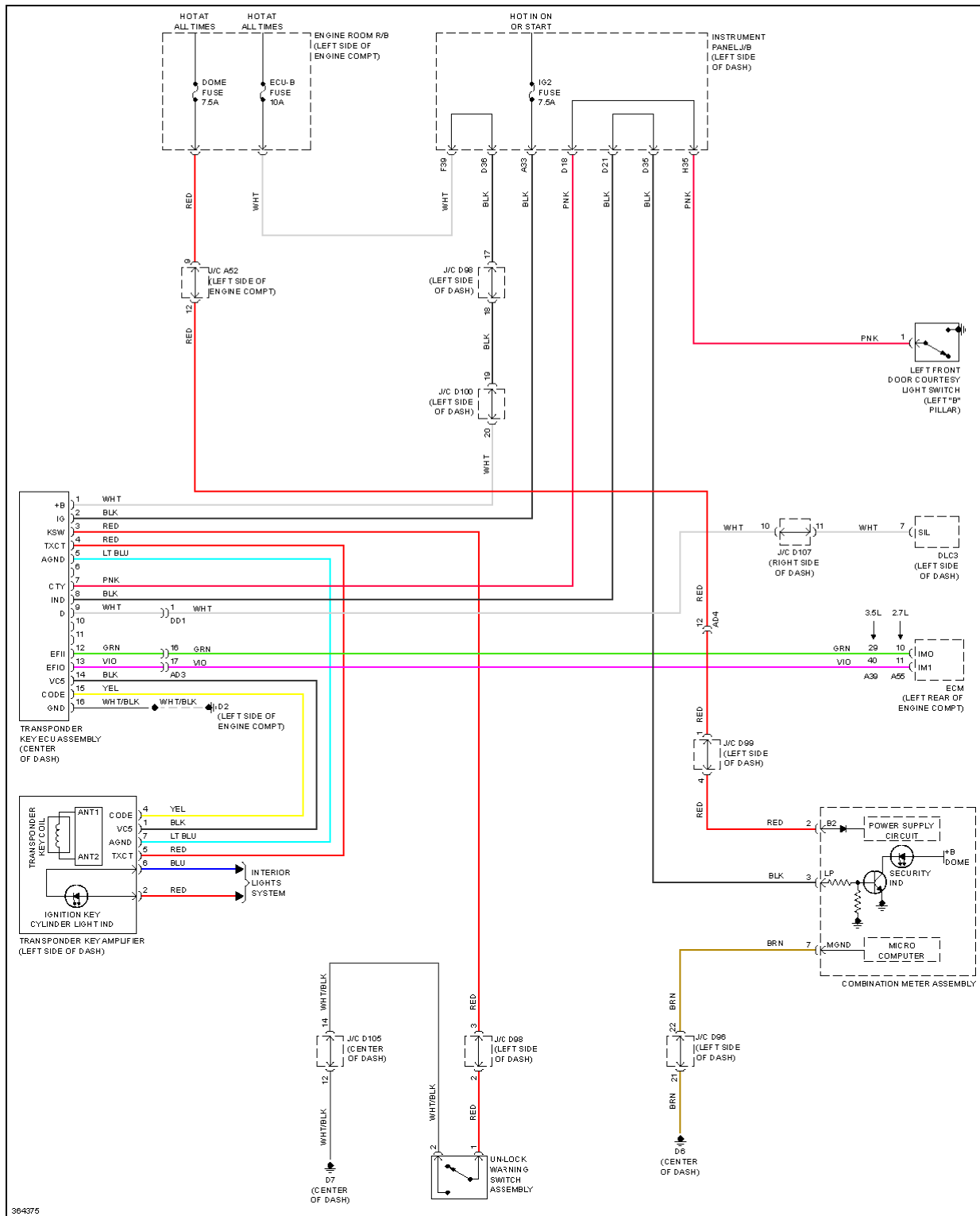
Fig. 12: Immobilizer Circuit, W/O Smart Key System
