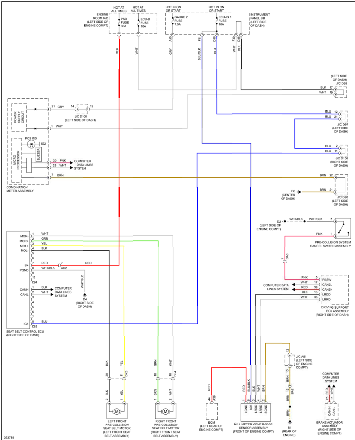
Fig. 108: Pre-Collision Circuit
