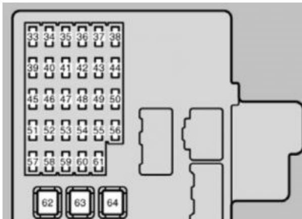
Lexus ES – fuse box – driver's side instrument
