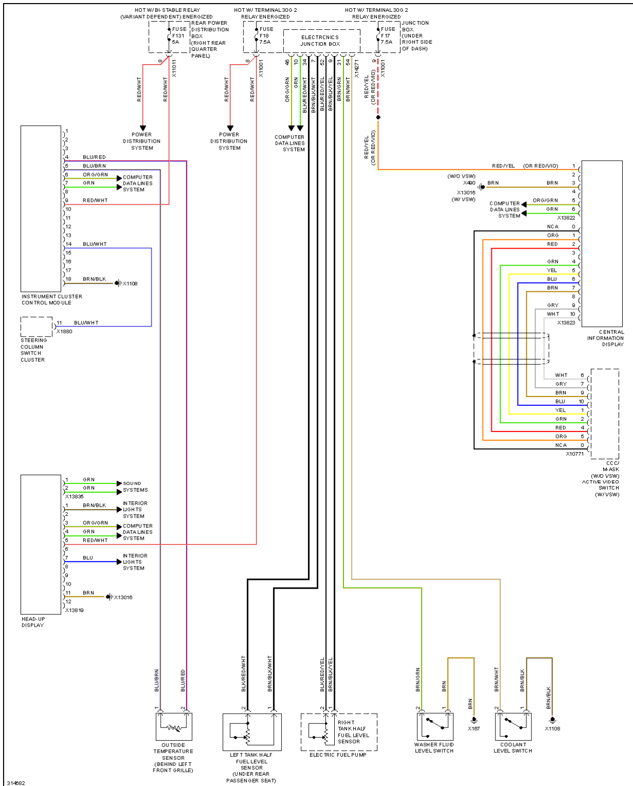
Fig. 56: Instrument Cluster Circuit
