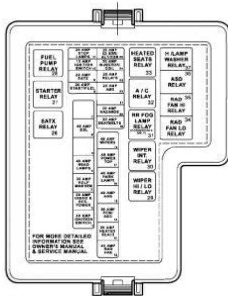
Dodge Stratus – fuse box –
