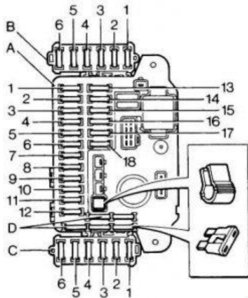
Land Rover Discover – fuse box diagram
