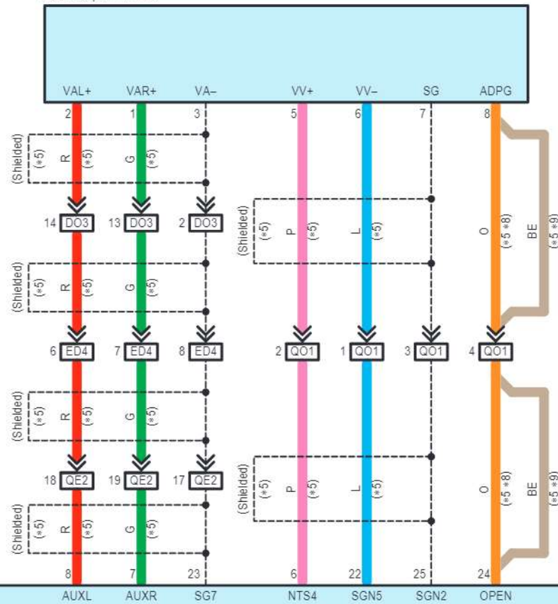
O25 Video Adapter Terminal
