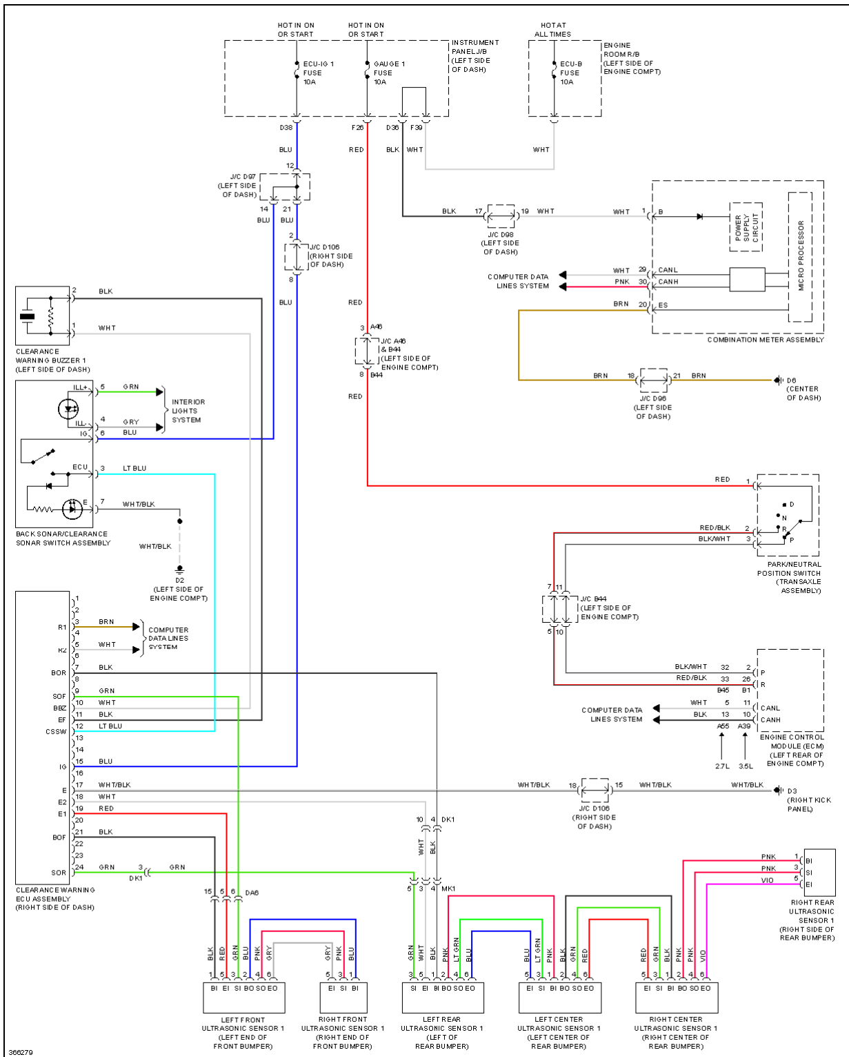
Fig. 66: Rear Sonar Circuit
