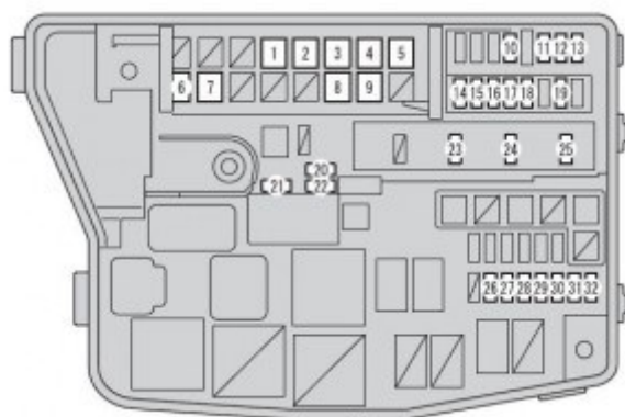
Scion xB mk2 – fuse box – engine compartment
