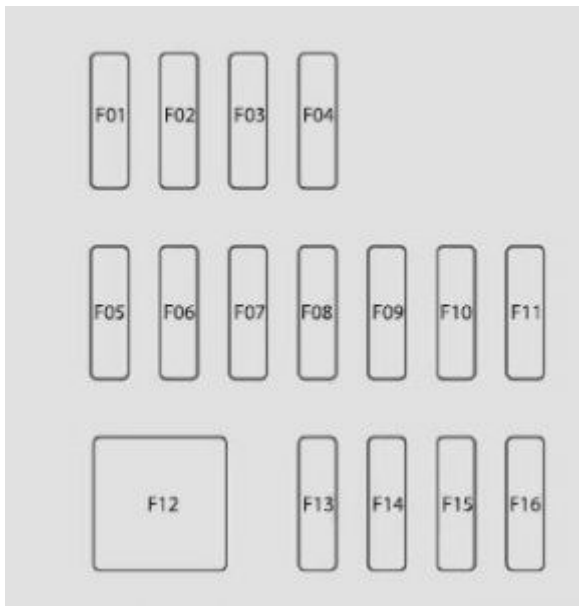
Fiat 124 Spider – fuse box diagram – left side
