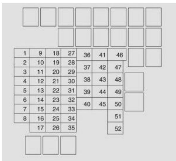
Fiat 124 Spider – fuse box diagram – engine
