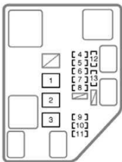
Scion xA – fuse box diagram – engine compartment
