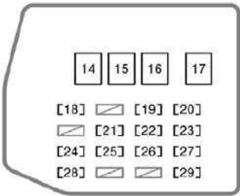
Scion xA – fuse box diagram – dashboard
