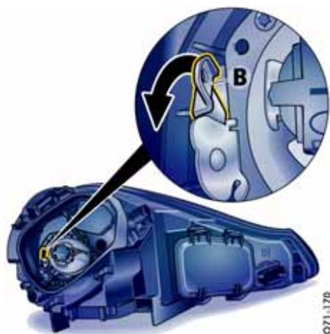
Halogen headlights
