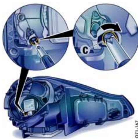
Xenon headlight
