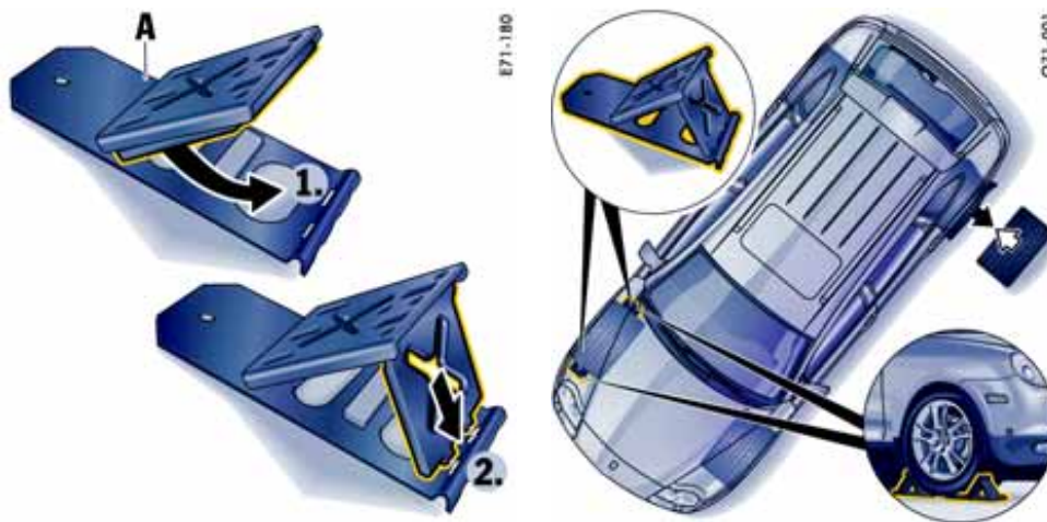
A - Folding wedges
