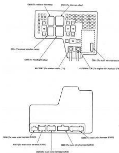
Isuzu Oasis – fuse box diagram – under-hood
