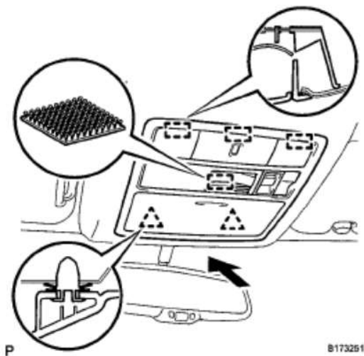
Fig. 13: Installing Roof Console Box Assembly, Clips And Guides Courtesy of TOYOTA MOTOR SALES, U.S.A., INC.
