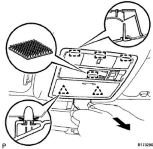
Fig. 12: Removing Roof Console Box Assembly, Clip, Claw And Guides Courtesy of TOYOTA MOTOR SALES, U.S.A., INC.
