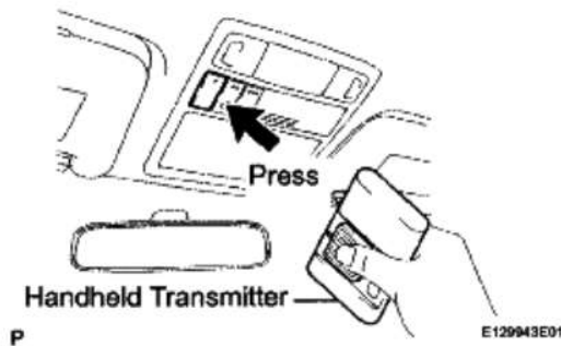
Fig. 9: Pressing And Holding Switch On Handheld Transmitter Courtesy of TOYOTA MOTOR SALES, U.S.A., INC.
