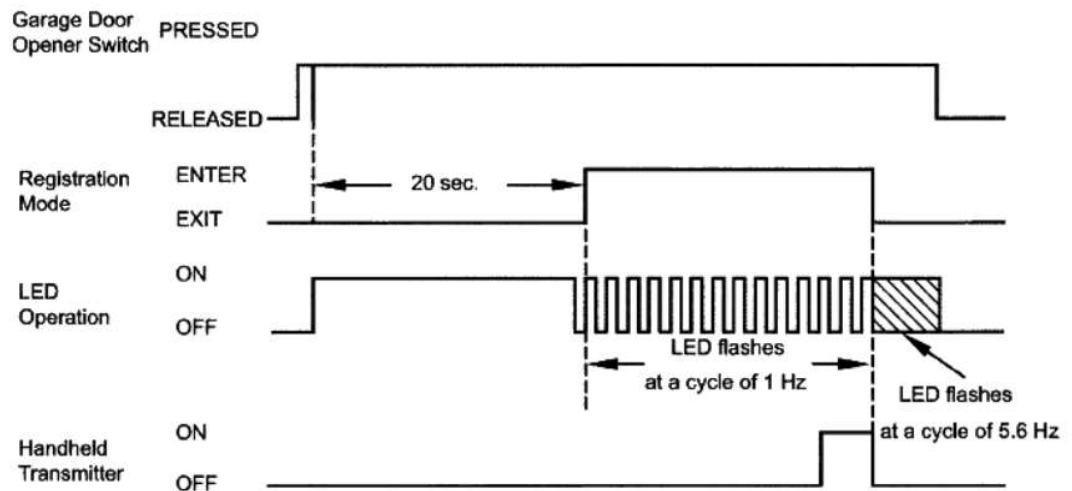
Fig. 6: Garage Door Opener Switch And Registration Mode Timing Pattern Courtesy of TOYOTA MOTOR SALES, U.S.A., INC.
