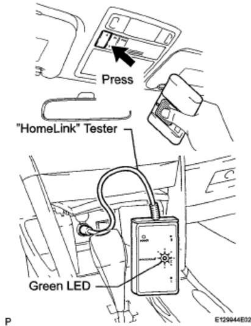
Fig. 10: Pressing Garage Door Opener Switch Courtesy of TOYOTA MOTOR SALES, U.S.A., INC.
