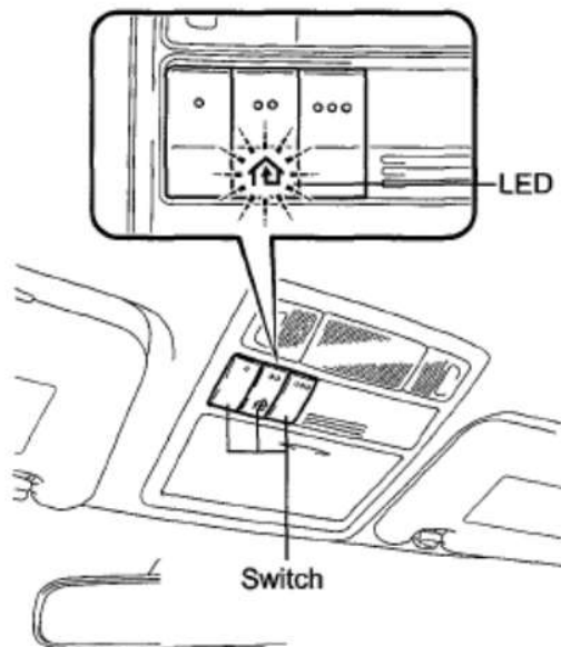
Fig. 8: Identifying Garage Door Opener System Switch Location Courtesy of TOYOTA MOTOR SALES, U.S.A., INC.
