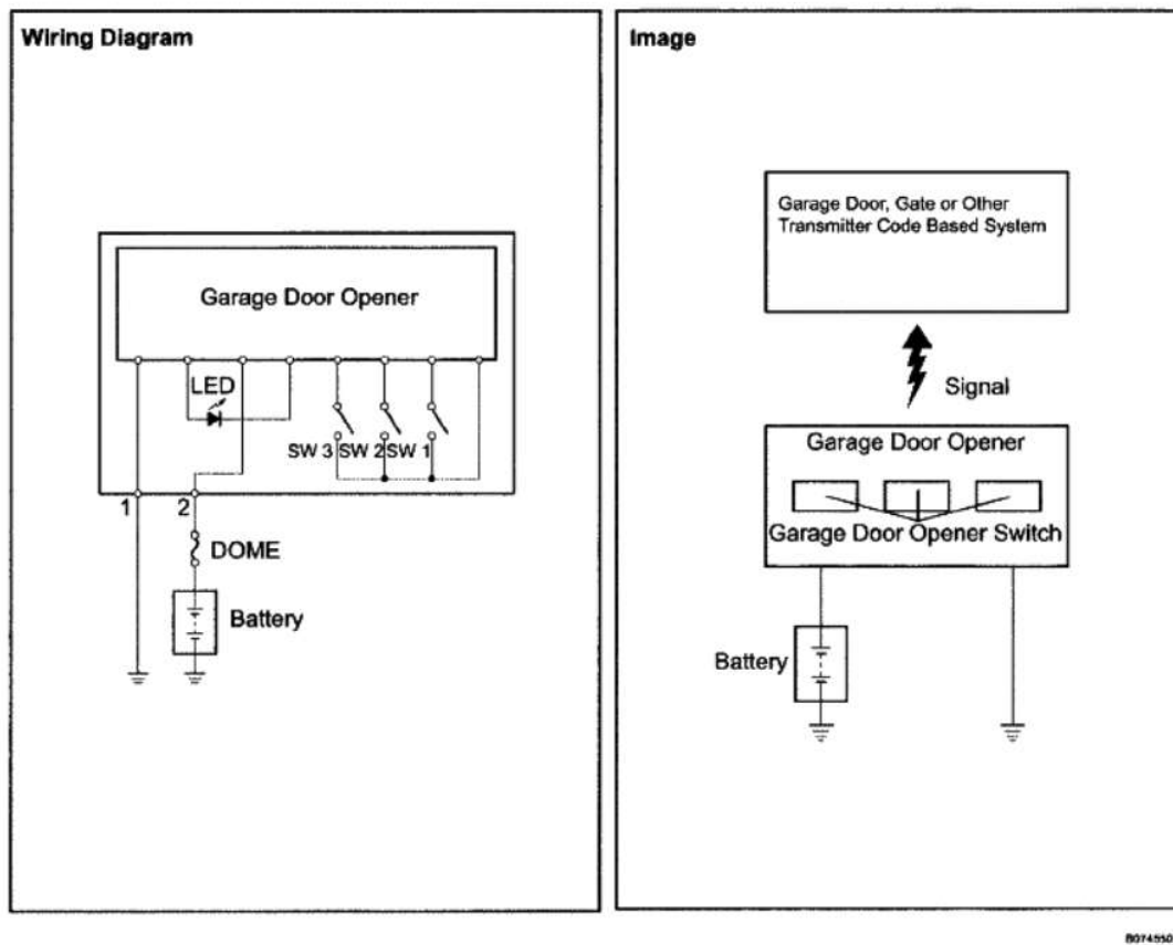
Fig. 1: Garage Door Opener System - Wiring Diagram Courtesy of TOYOTA MOTOR SALES, U.S.A., INC.
