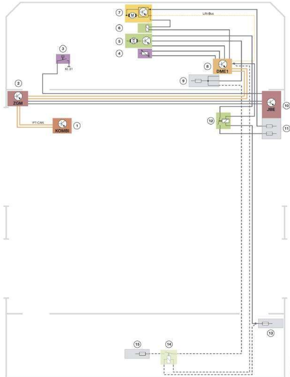
N55, circuit diagram, engine cooling
